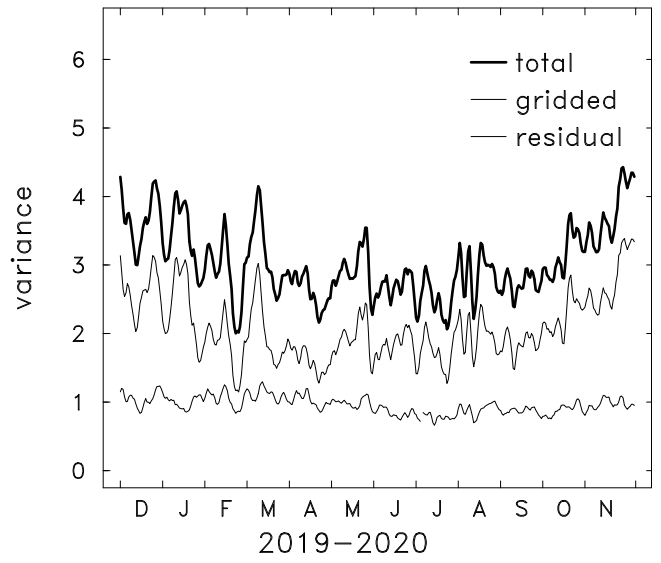
H2O variance 5km 8-8
