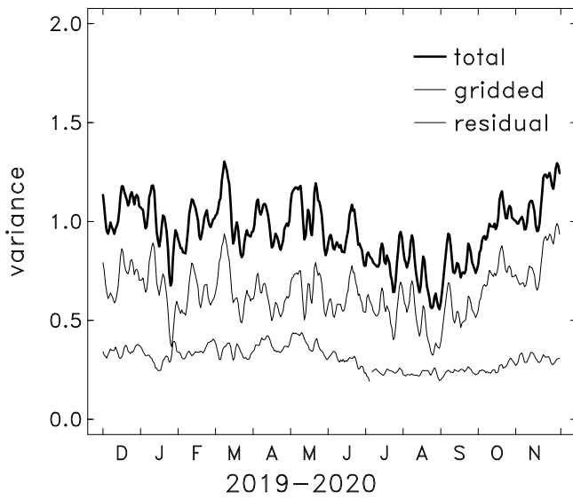
H2O variance 7km 8-8
