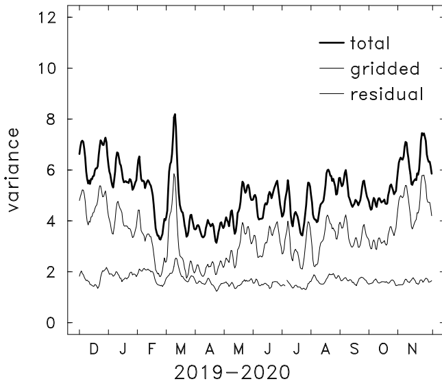
H2O variance 3km 8-8
