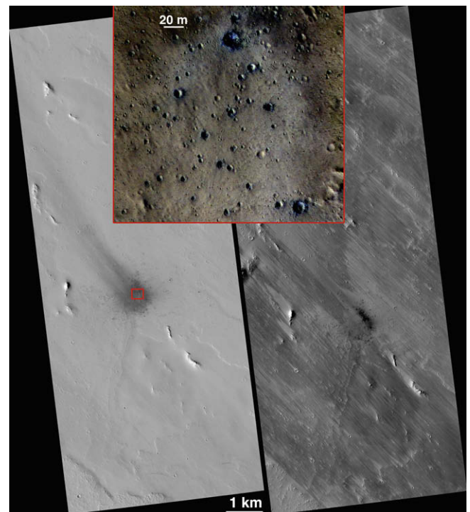
Fig. 13. A large new impact cluster in PSP_003172_1870 (left and full-resolution false-color inset) and PSP_007431_1870 (right). These images were acquired before and after the global-scale dust storms of 2007, and show that fresh and relatively dark impact markings can disappear by darkening of the surroundings from dust removal as well as from new dust deposition that homogenizes the albedo. Thousands of new small impact craters were created by this single event. Several other new impact sites imaged before and after the 2007 dust storms do not show obvious changes.
