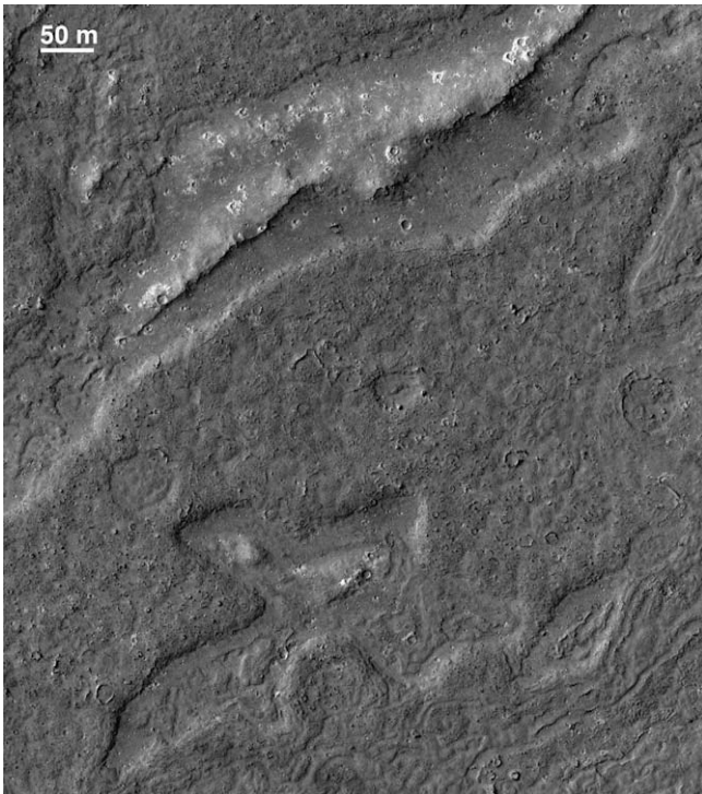
Fig. 15. Example of inflated lavas in the western margin of the Cerberus Palus lava flow that erupted from the head of Athabasca Valles, ~850 km to the east-northeast. Thin lobes of lava flowed around topographic obstacles, then inflated vertically, often to greater heights than the original obstacles. The many small bright-ejecta craters over areas not covered by the young lava are secondary craters from the rayed crater Corinto, ~735 km almost directly north of this location. Corinto rays are superimposed on this lava flow, but the detectability and retention of small craters varies with physical properties of the surfaces. PSP_007448_1845, equirectangular projection (north is up); illumination from the west (left).
