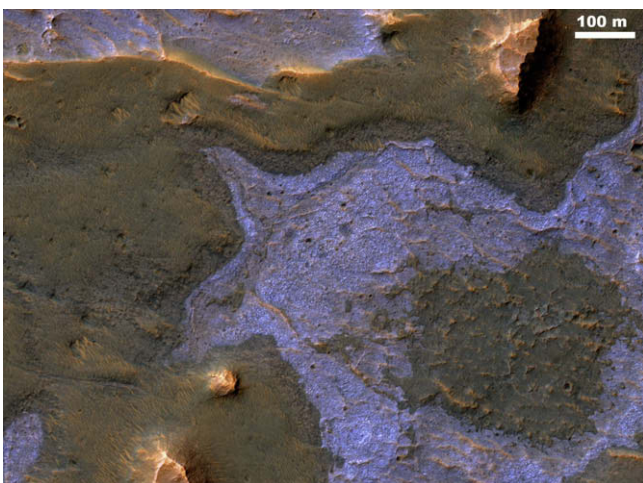
Fig. 12. Section of PSP_008780_1735. This image was acquired of a site suggested by the THEMIS team as having exposed chloride salts. This color composite shows distinct surface units. At the highest resolution, the apparently blue material shows a cracked surface structure.
