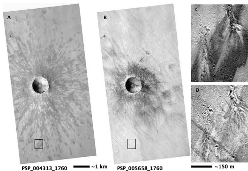
Fig. 14. HiRISE images of Winslow crater, showing changes before and after the dust storms of 2007. North is up in these equirectangular projections.
