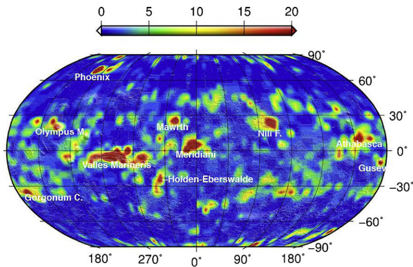
Fig. 2. Map of HiRISE imaging coverage density near end of PSP: number of images in 5 \times 5 latitude/longitude bins (not normalized for area). This scale saturates at 20 images, but the most populous bins have >100 images in them. Frequently imaged locations include the Phoenix landing ellipse, Olympus Mons, Gorgonum Chaos, and other mid-latitude regions, Valles Marineris and surrounding plains, Mawrth Vallis region, Meridiani Planum, Holden and Eberswalde craters, the Nili Fossae region, Athabasca Valles, and Gusev crater. Both polar regions are also densely covered by HiRISE images, but that is disguised by the map projection.
