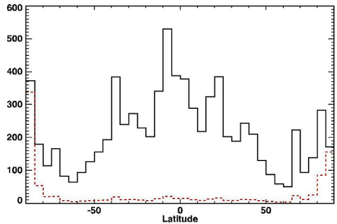
Fig. 3. Histogram of number of images in bins of 5^\circ of latitude; the dashed red curve shows the same histogram normalized for area (images per quarter million \text{km}^2 as a function of latitude). Same dataset as that used for Fig. 2.
