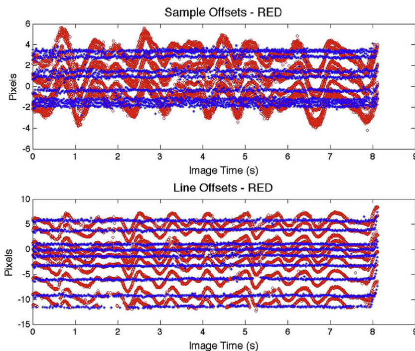
Fig. 10. Coregistration data from all nine of the overlapping RED CCD pairs in PSP_007124_1765 plotted from before jitter removal (red) and after jitter removal (blue). Sample and line offsets are measured in pixels and plotted against the image time in seconds. Data points are extracted every 50 lines. The high-frequency distortions have been removed by the jitter correction algorithm, except near the very ends of the image. The average offset of each CCD pair is preserved, and is a function of the camera geometry. (For interpretation of color mentioned in this figure the reader is referred to the web version of the article.)
