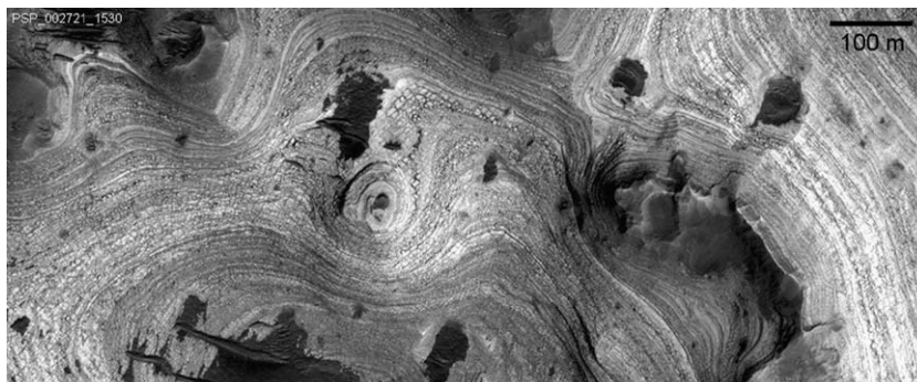
Fig. 19. Portion of HiRISE image PSP_002721_1530 in Holden crater showing sub-meter thick and laterally continuous beds of the upper member of the lower unit. Characteristics of these deposits discernable in HiRISE images enable their depositional setting to be constrained to a distal alluvial or lacustrine aqueous environment.
