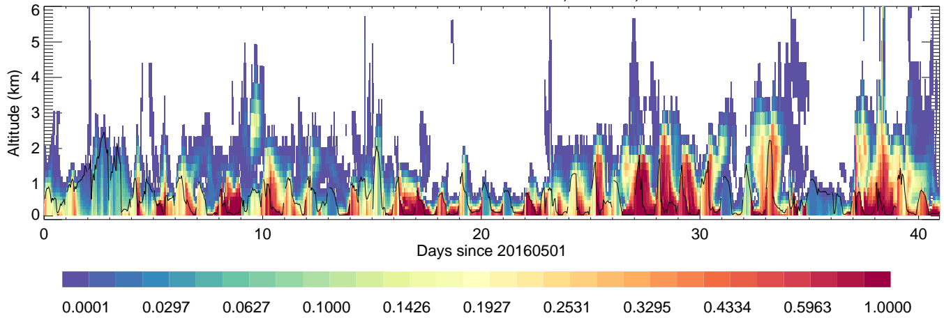
UlsanUNIST: AreaMobile,unitless,
