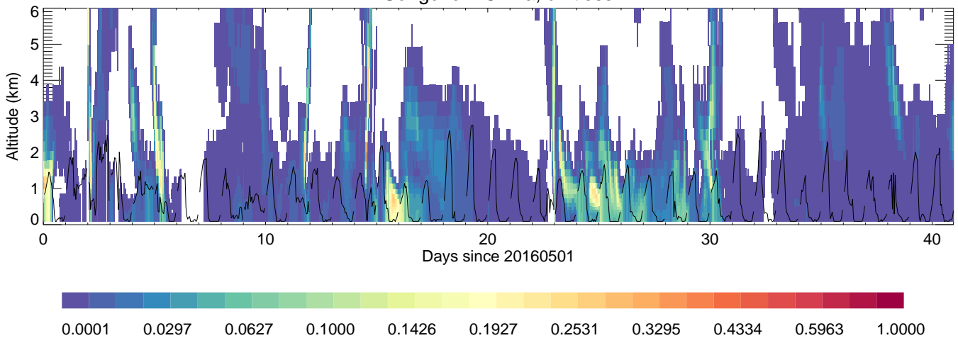
Songchon: China,unitless
