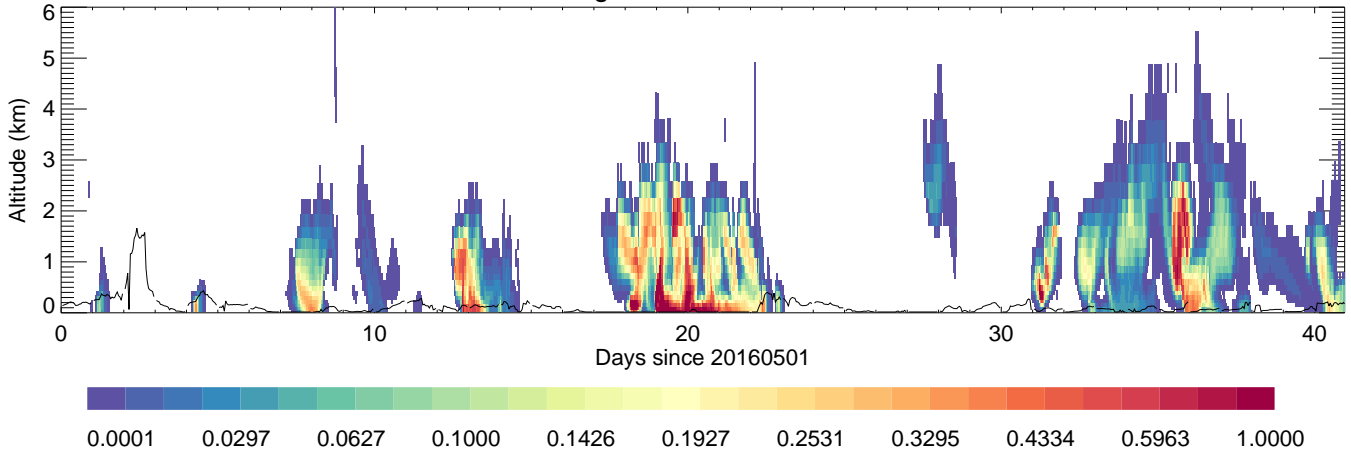
Socheongcho: AreaMobile,unitless,
