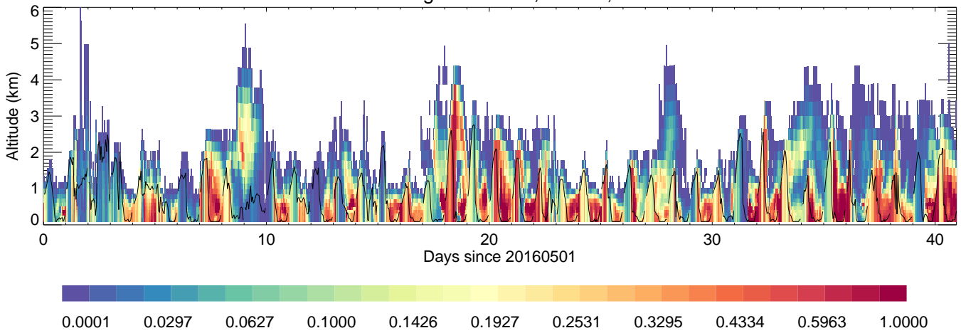
Songchon: China,unitless
