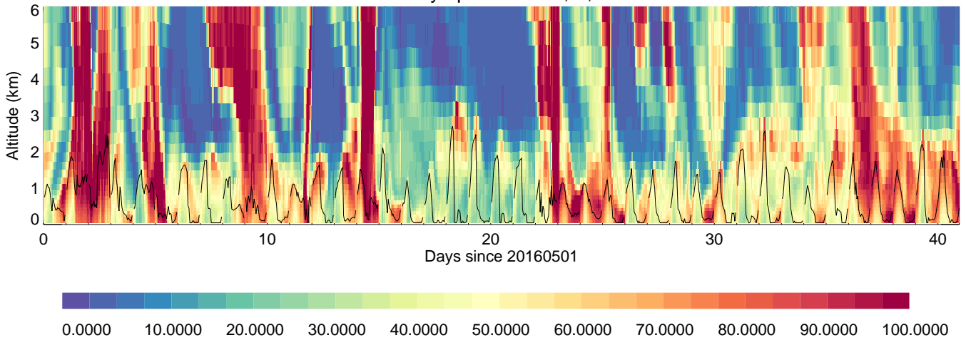
OlympicPark: RH,%,
