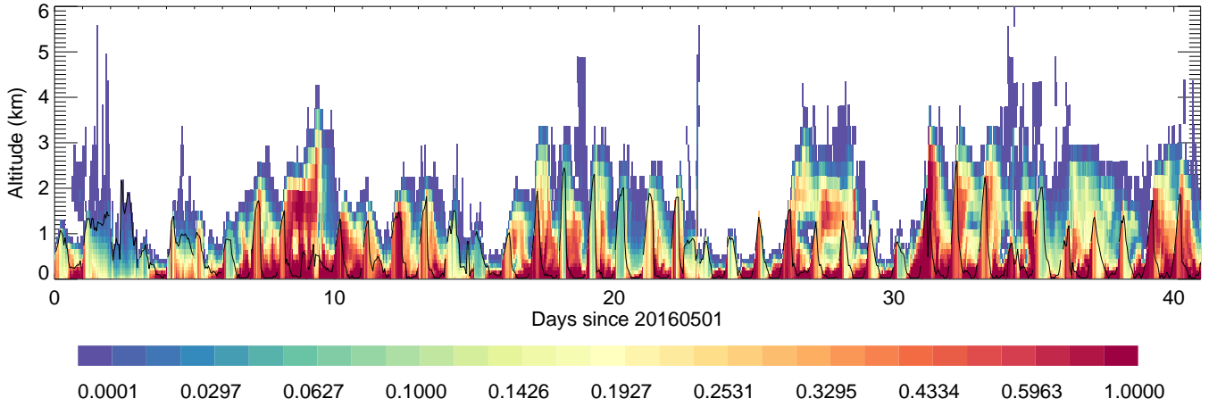
Iksan: AreaMobile,unitless,
