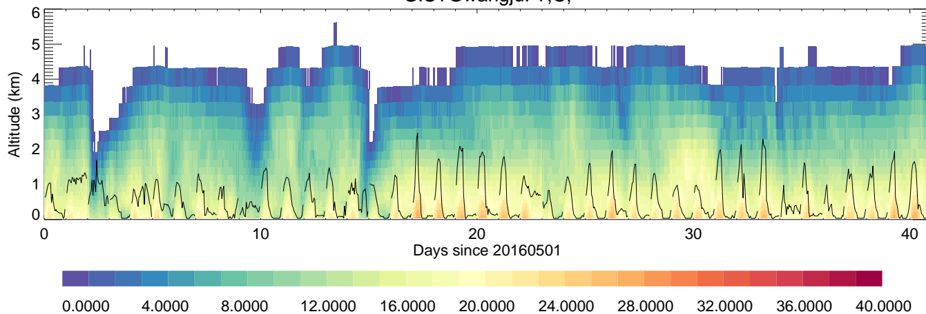
GISTGwangju: T,C,
