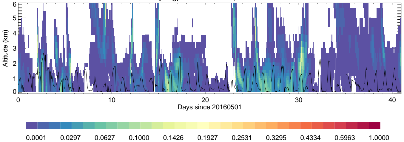
KyungpookNU: China,unitless
