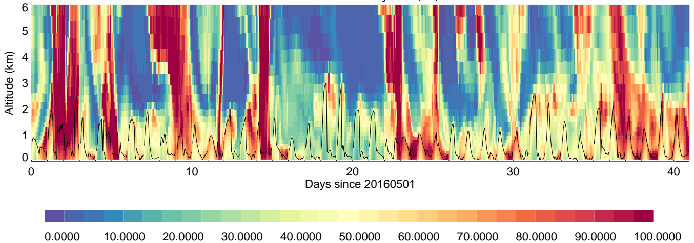
YonseiUniversity: RH, %,
