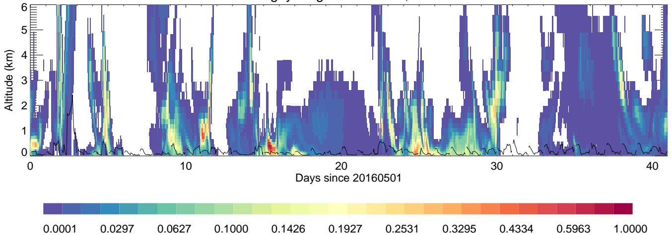
BaengnyeongIsland: China,unitless
