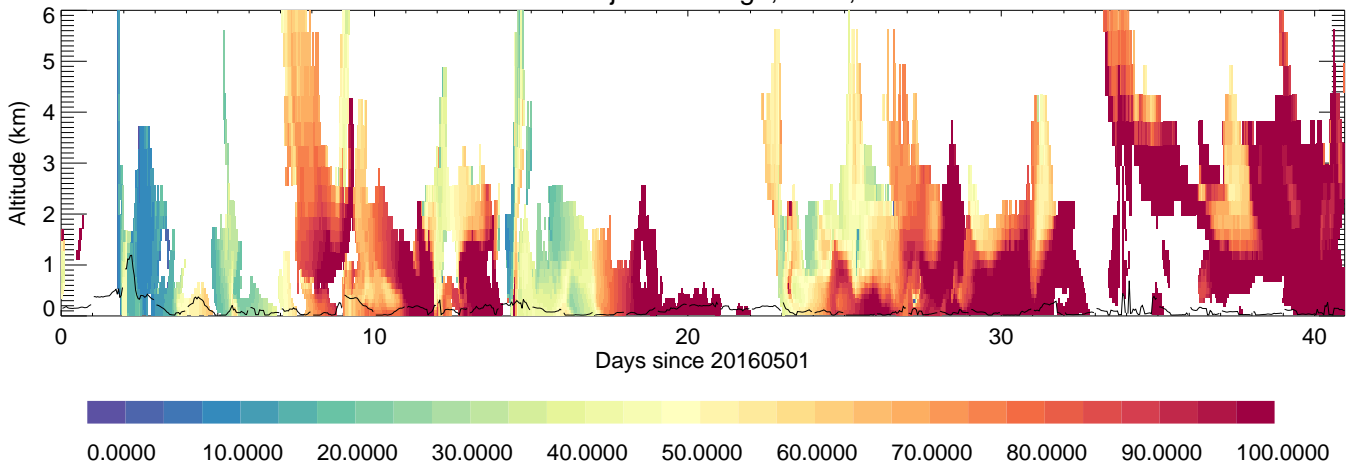
Jeonju: RH,%,
