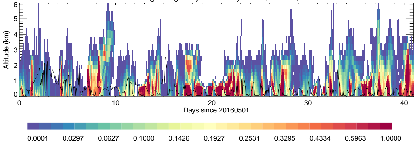
GangneungWonjuUniversity: China,unitless
