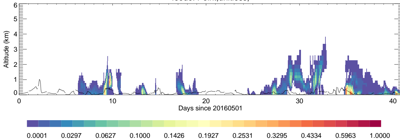
leodo: Point,unitless,
