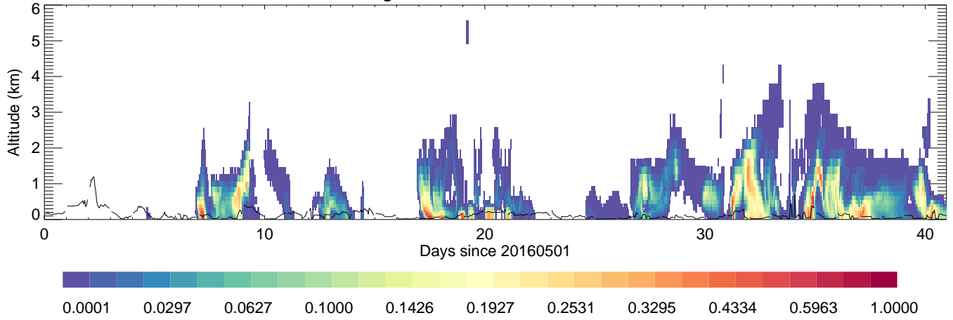
Gagecho: AreaMobile,unitless,
