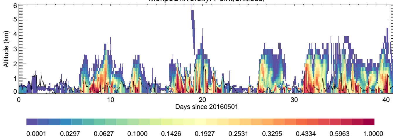
MokpoUniversity: Point,unitless,
