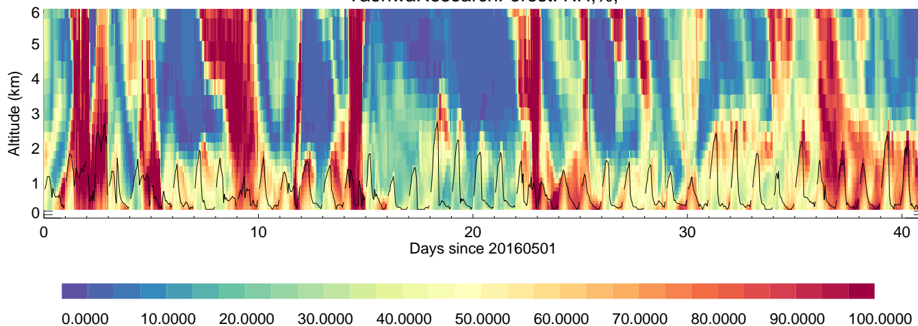
TaehwaResearchForest: RH, %,
