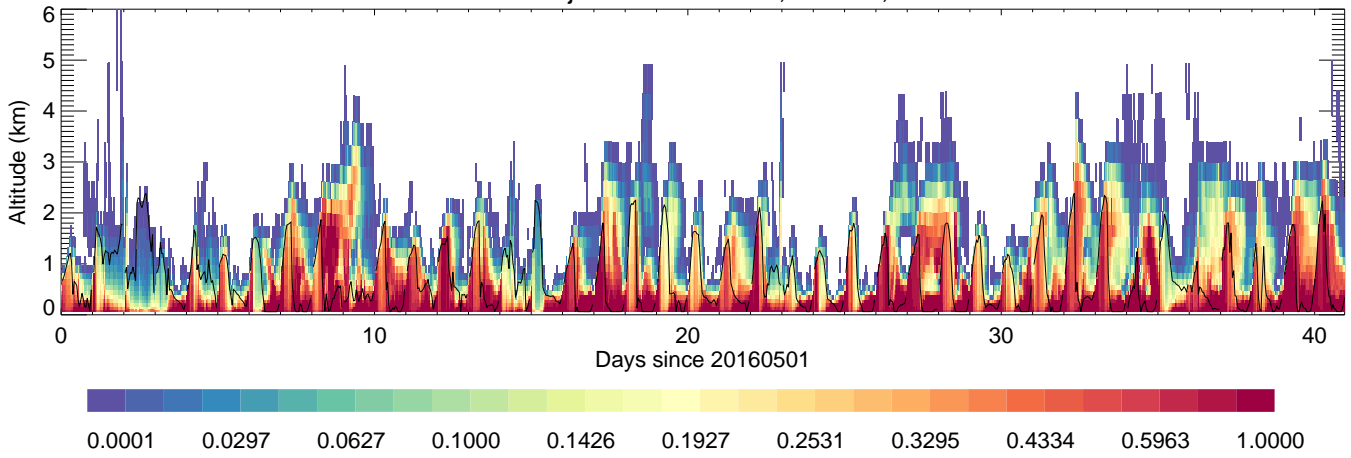
Daejeon: AreaMobile,unitless,
