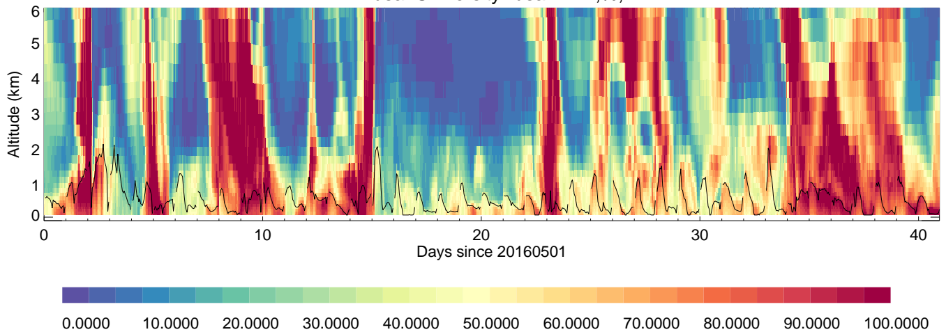
PusanUniversityBusan: RH,%,
