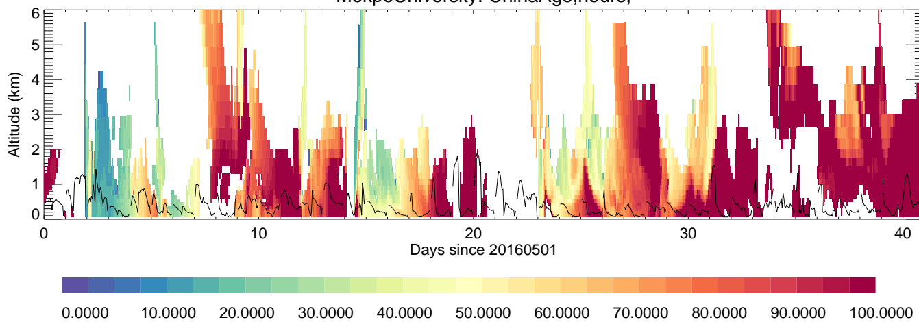
MokpoUniversity: RH, %,
