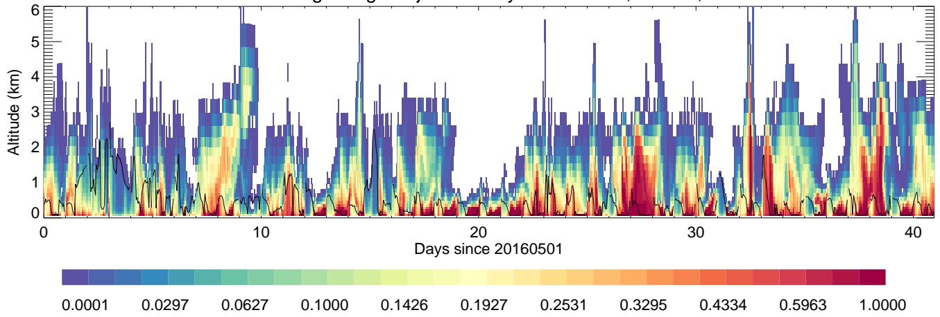
GangneungWonjuUniversity: AreaMobile,unitless,
