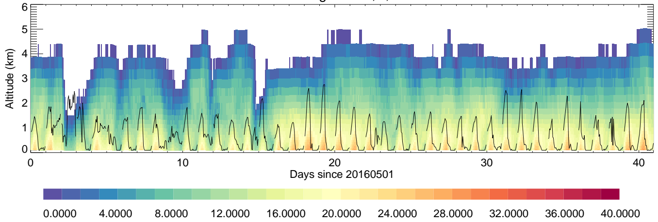
Songchon: T,C,
