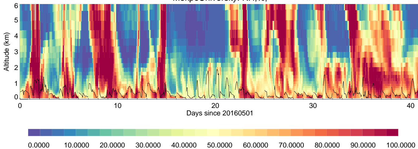
MokpoUniversity: RH, %,
