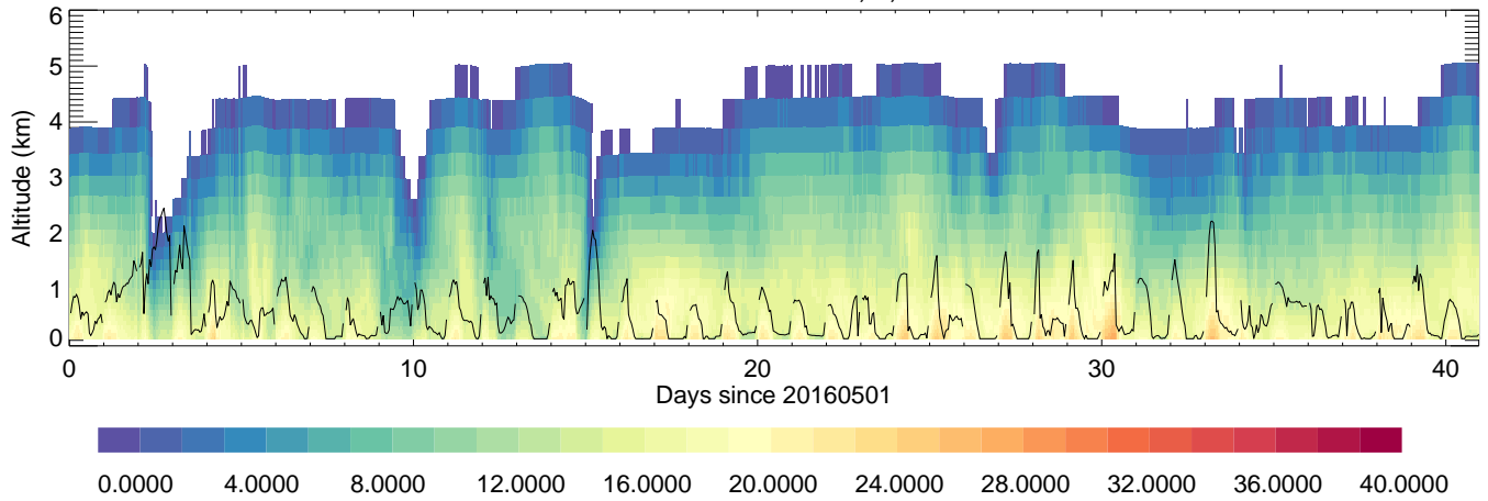
UlsanUNIST: T,C,
