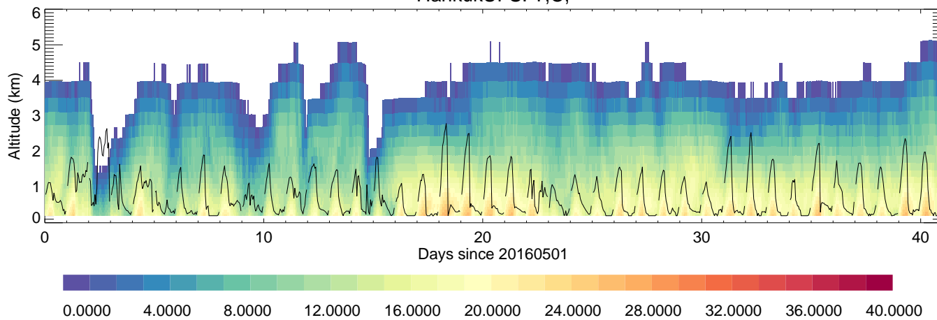
HankukUFS: T,C,
