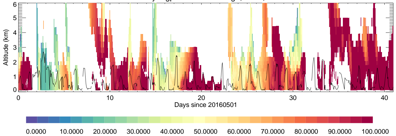
KyungpookNU: RH,%,
