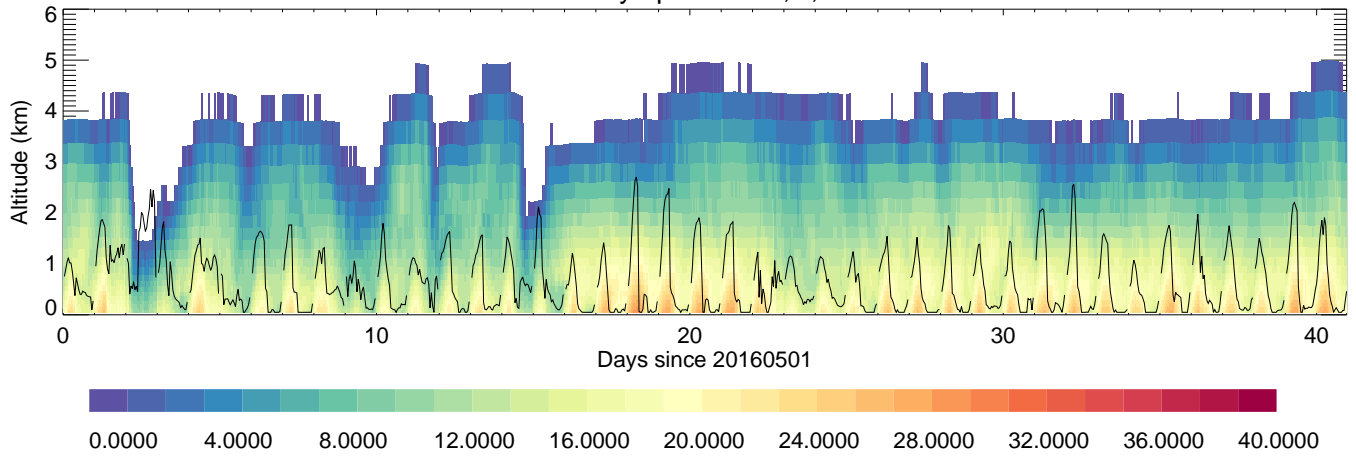
OlympicPark: T,C,
