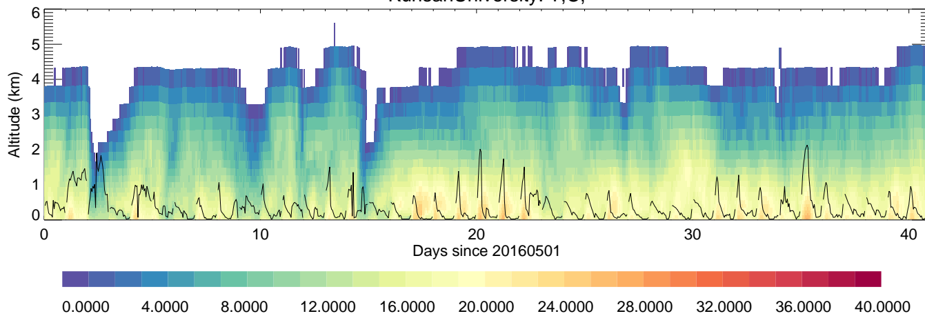
KunsanUniversity: T,C,
