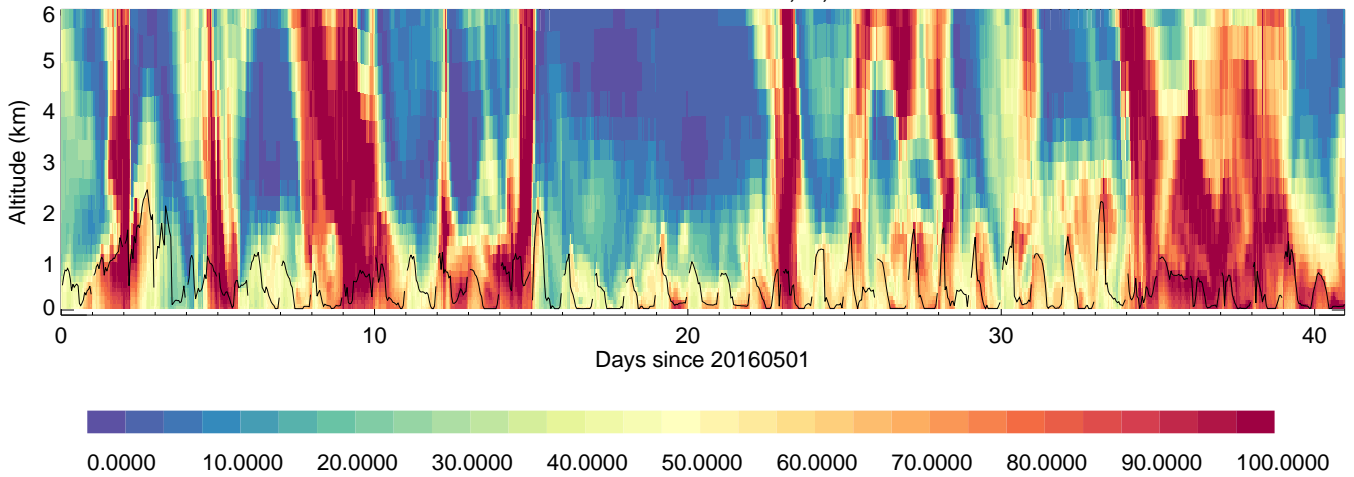
UlsanUNIST: RH,%,
