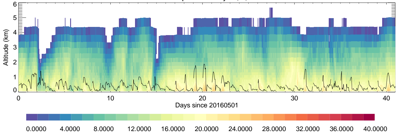
MokpoUniversity: T,C,
