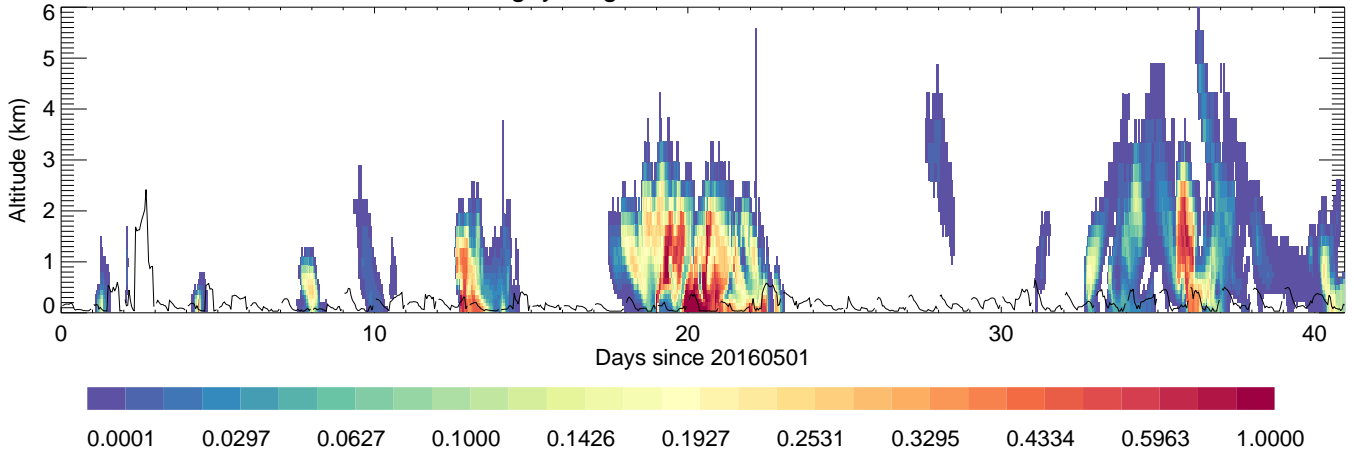
BaengnyeongIsland: AreaMobile,unitless,
