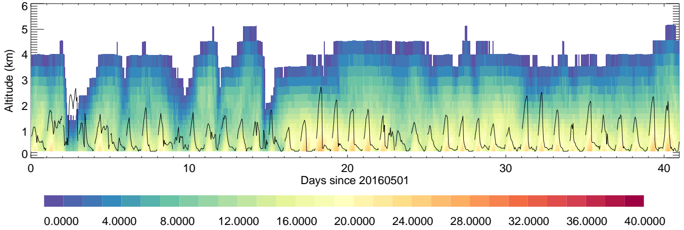
TaehwaResearchForest: T,C,
