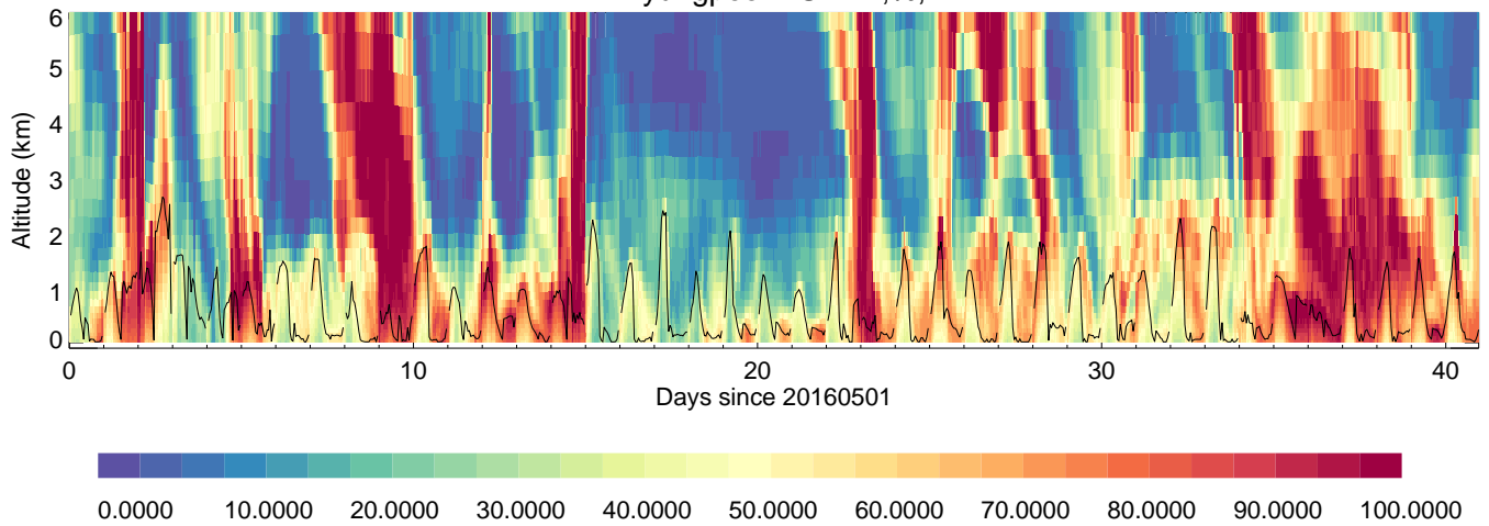
KyungpookNU: RH,%,
