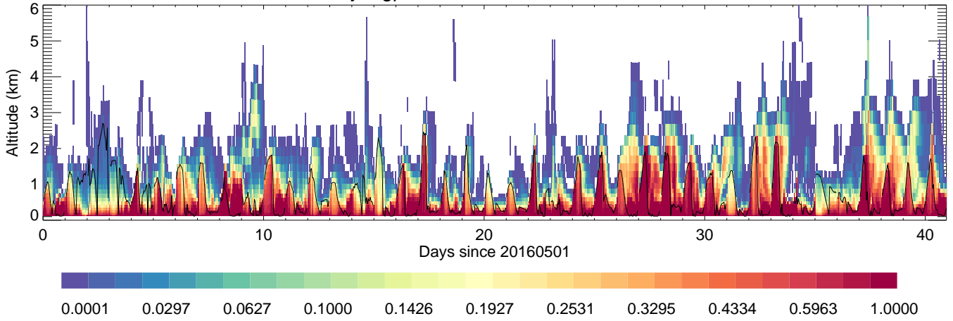
KyungpookNU: AreaMobile,unitless,
