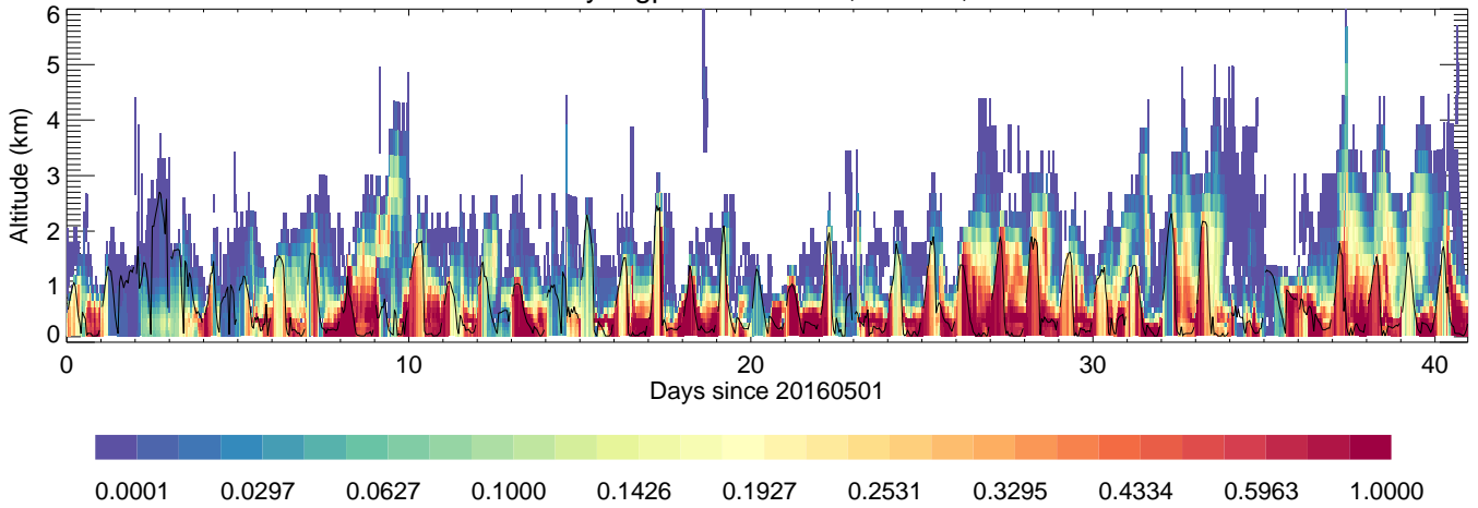
KyungpookNU: China,unitless
