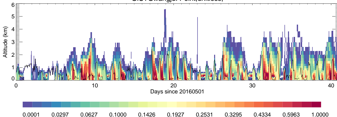
GISTGwangju: Point,unitless,
