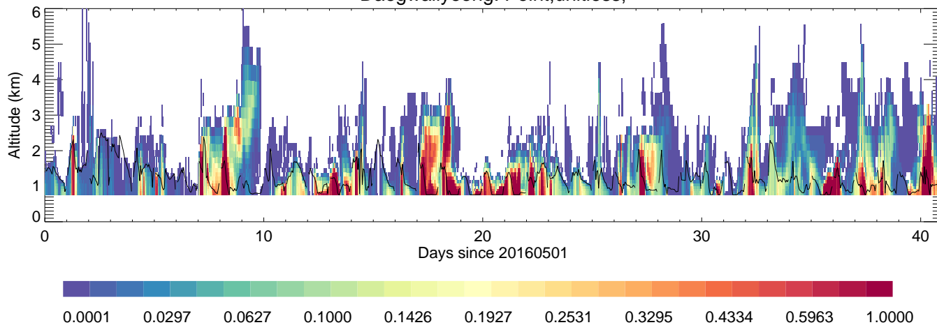
Daegwallyeong: Point,unitless,
