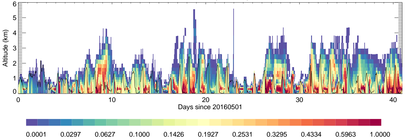
Iksan: Point,unitless,
