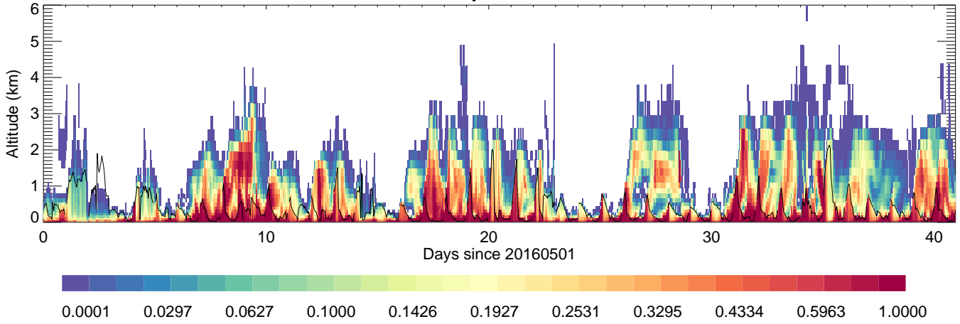
KunsanUniversity: AreaMobile,unitless,
