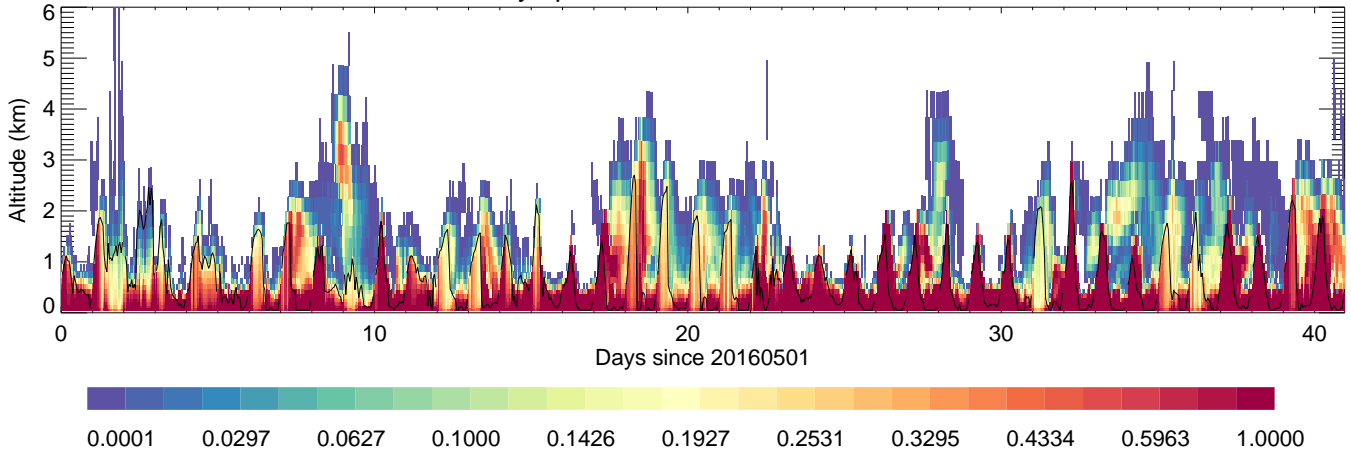
OlympicPark: AreaMobile,unitless,
