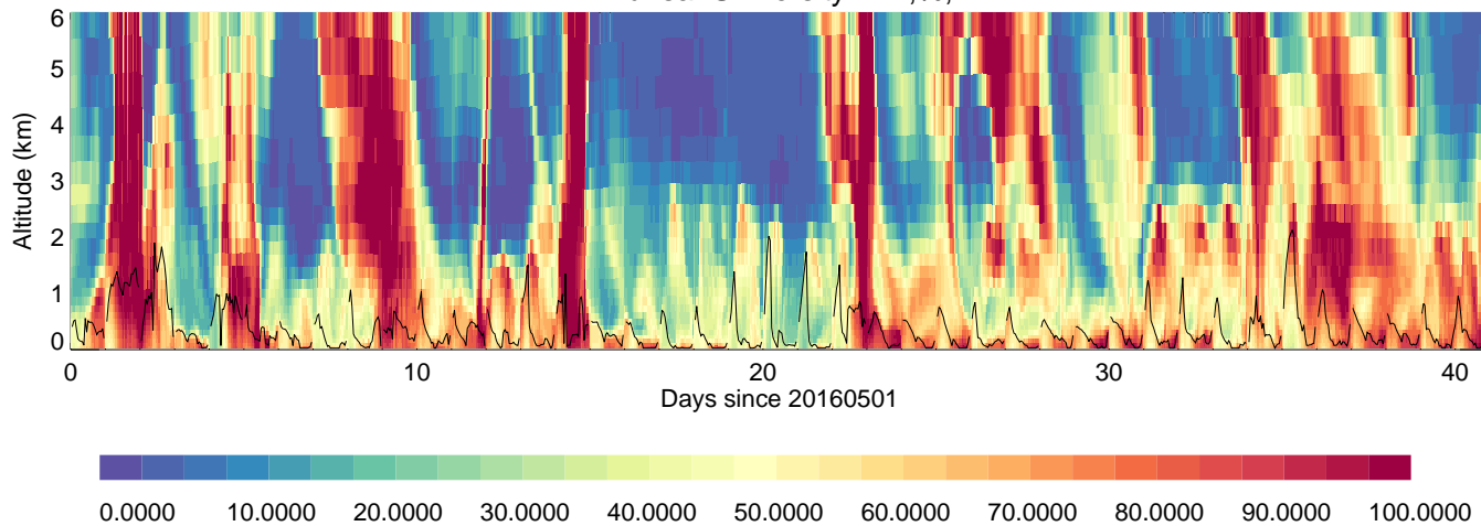
KunsanUniversity: RH,%,
