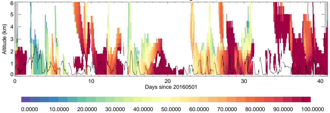
UlsanUNIST: RH,%,
