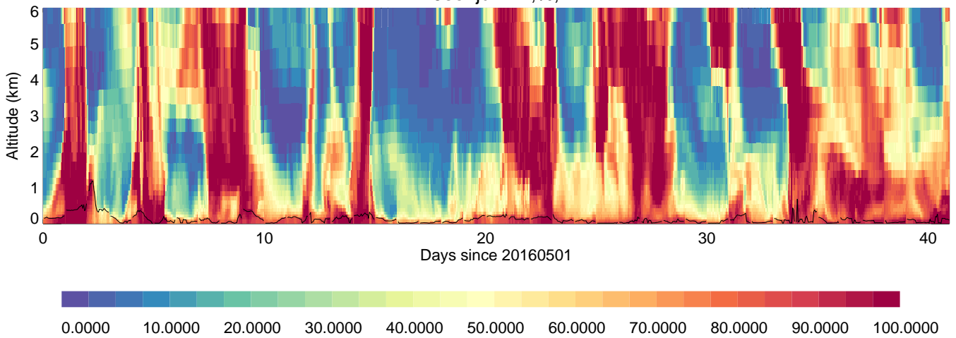
Jeonju: RH,%,
