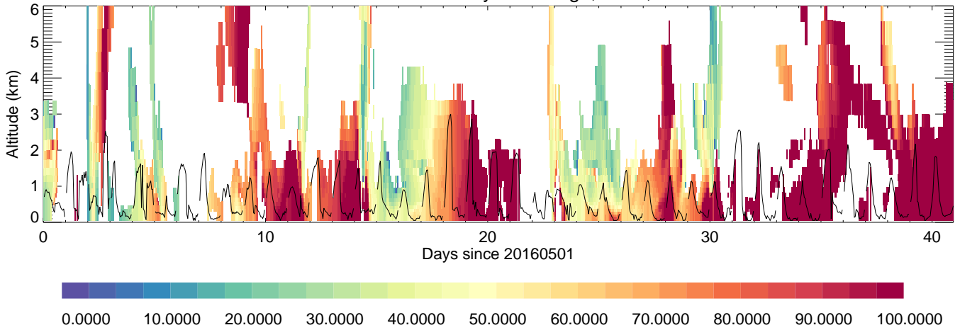
YonseiUniversity: RH, %,
