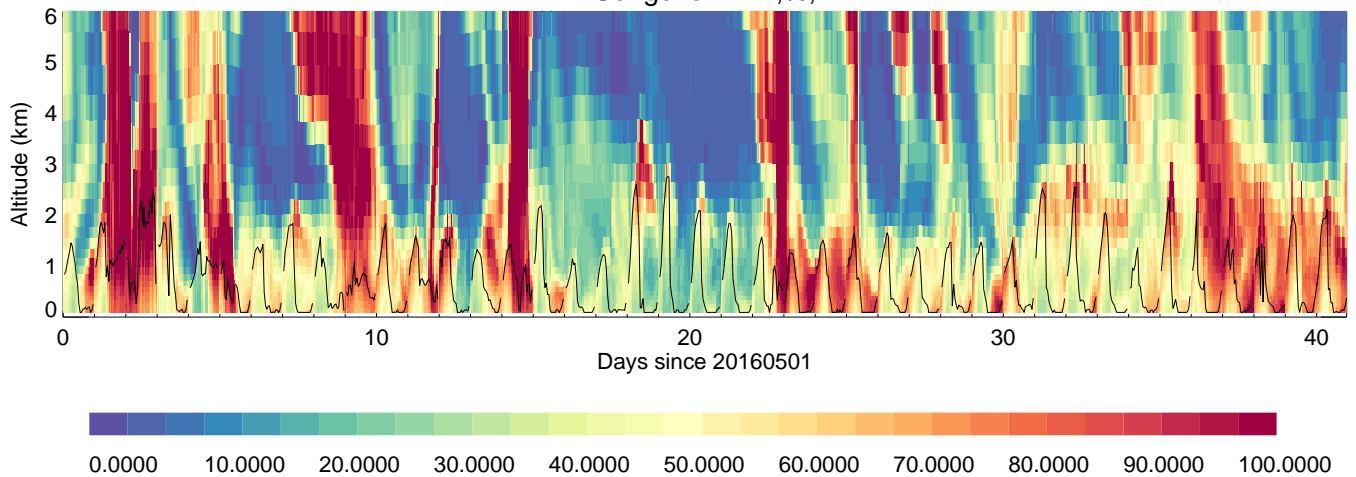
Songchon: RH,%,
