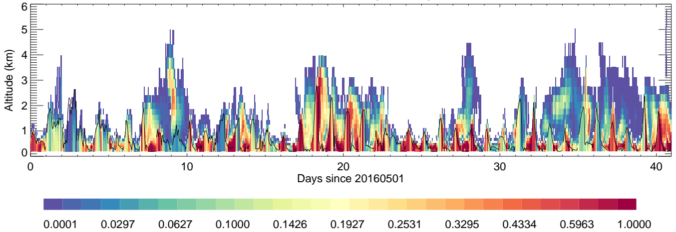
SeoulSNU: Point,unitless,
