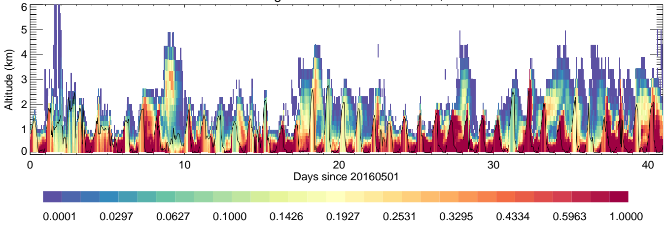
Songchon: AreaMobile,unitless,
