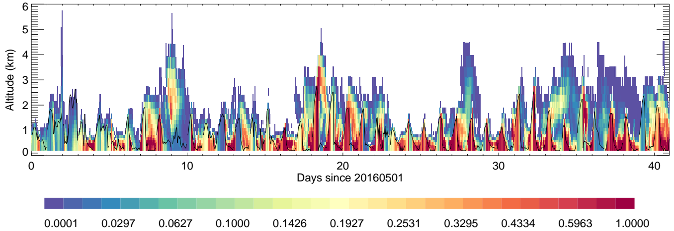
HankukUFS: Point,unitless,
