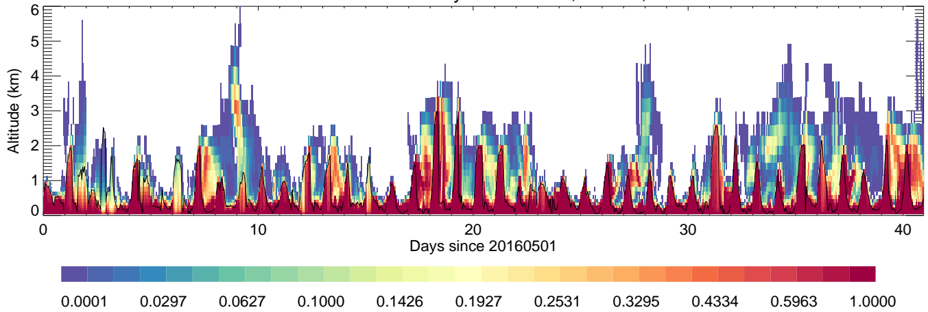
YonseiUniversity: AreaMobile,unitless,
