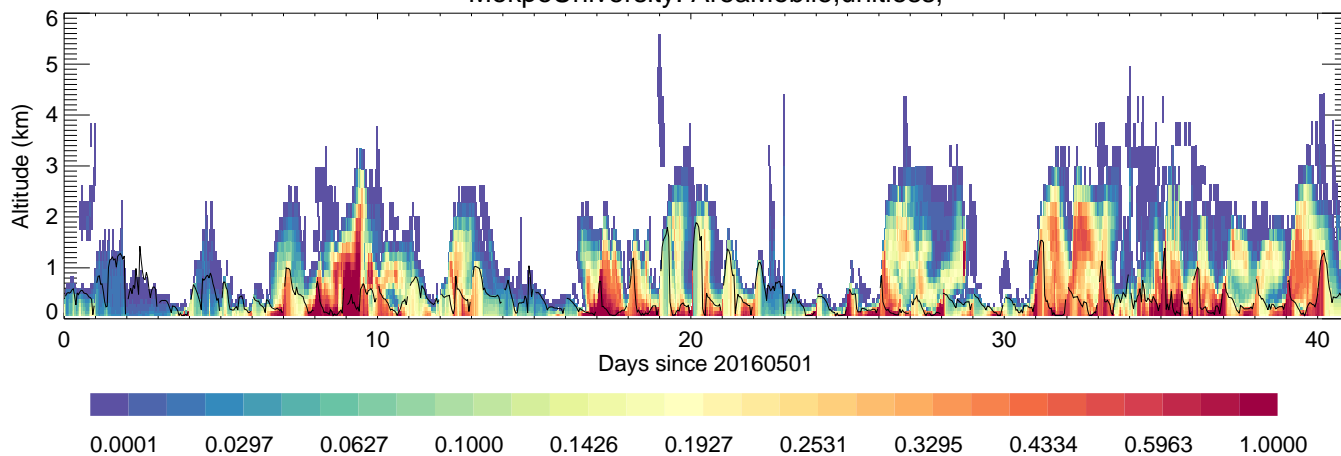
MokpoUniversity: AreaMobile,unitless,
