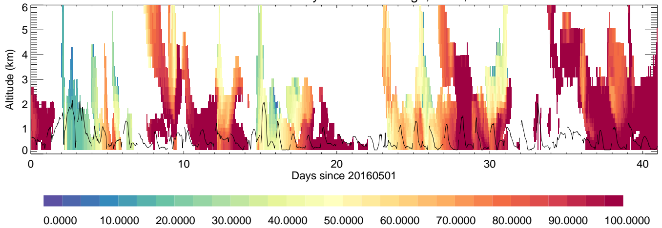
PusanUniversityBusan: RH,%,
