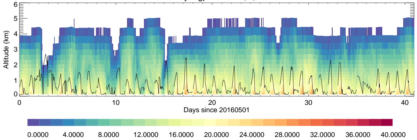
KyungpookNU: T,C,
