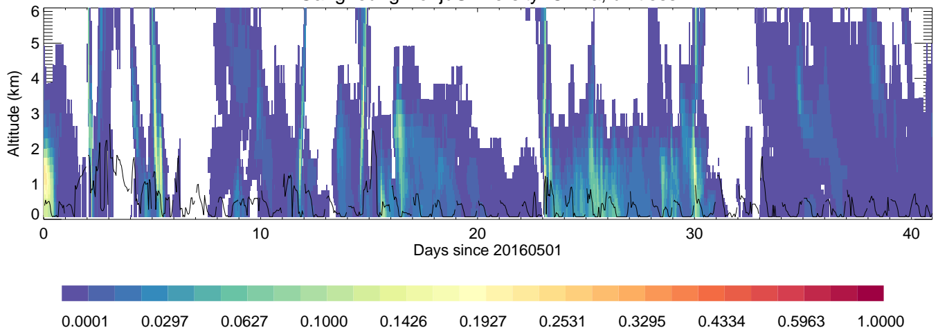
GangneungWonjuUniversity: China,unitless
