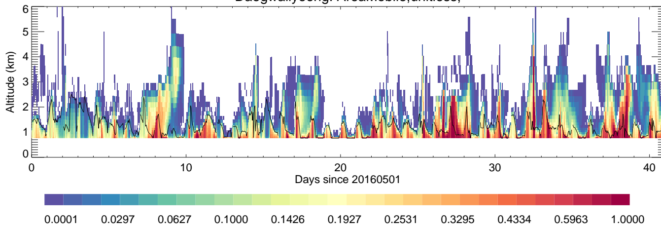
Daegwallyeong: AreaMobile,unitless,
