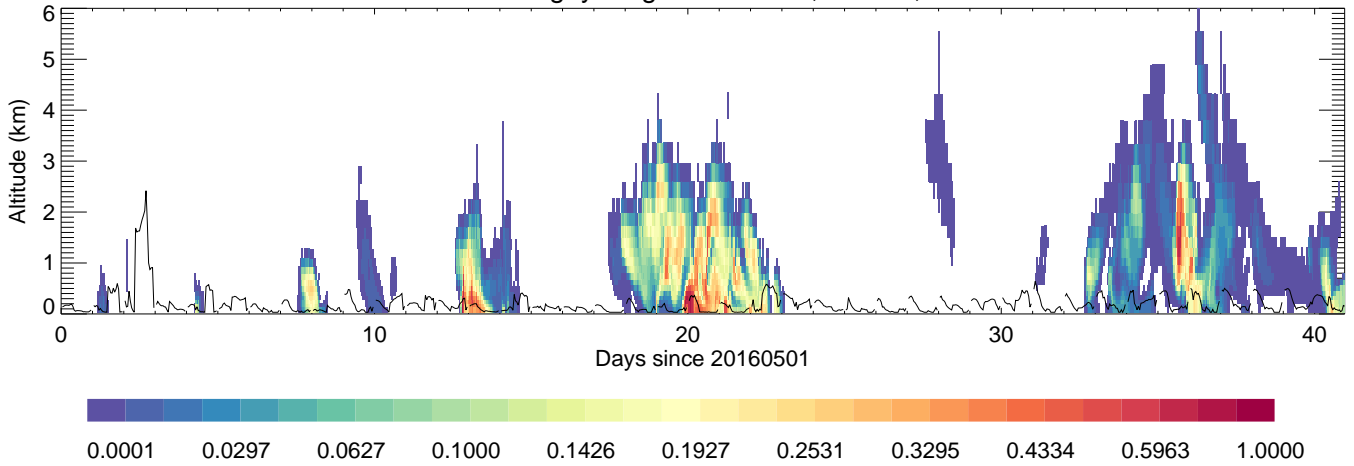
BaengnyeongIsland: China,unitless
