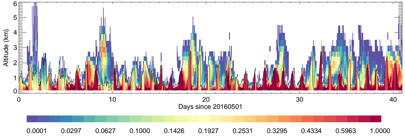
HankukUFS: AreaMobile,unitless,
