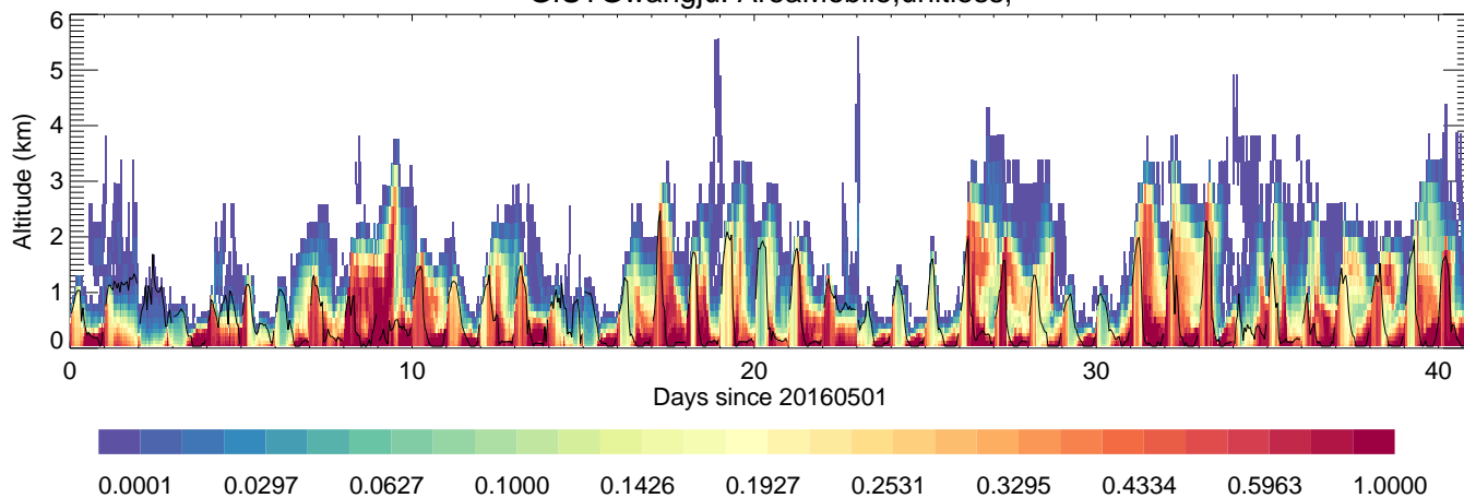
GISTGwangju: AreaMobile,unitless,
