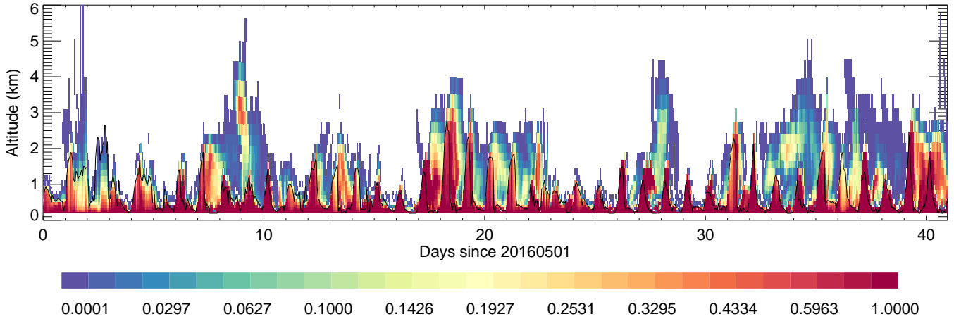
SeoulSNU: AreaMobile,unitless,
