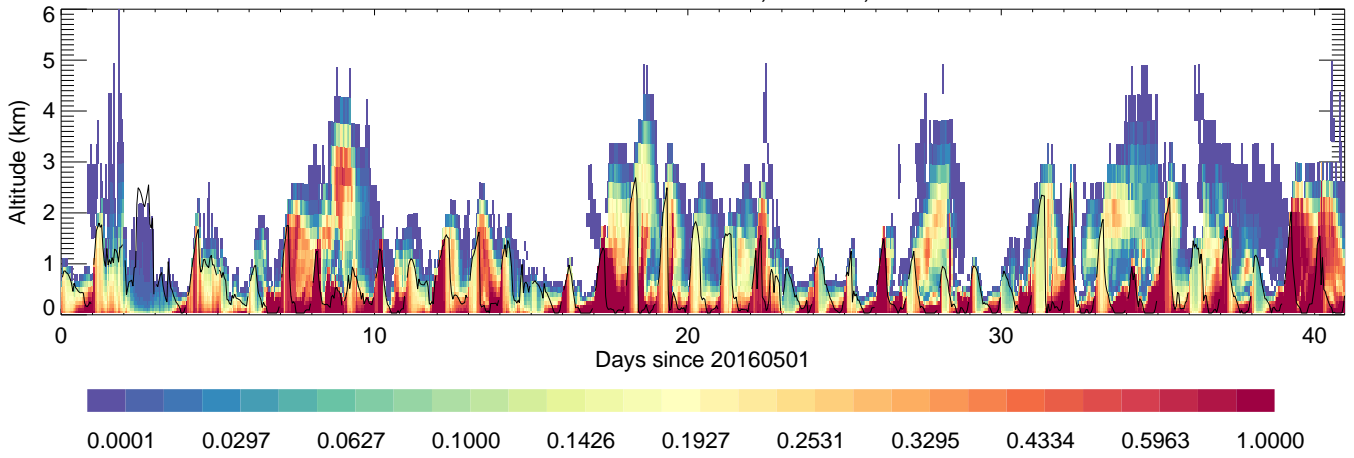
Osan: AreaMobile,unitless,
