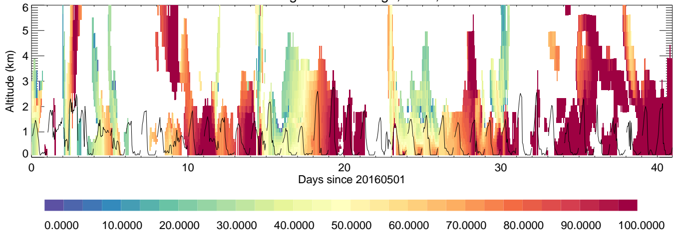
Songchon: RH,%,
