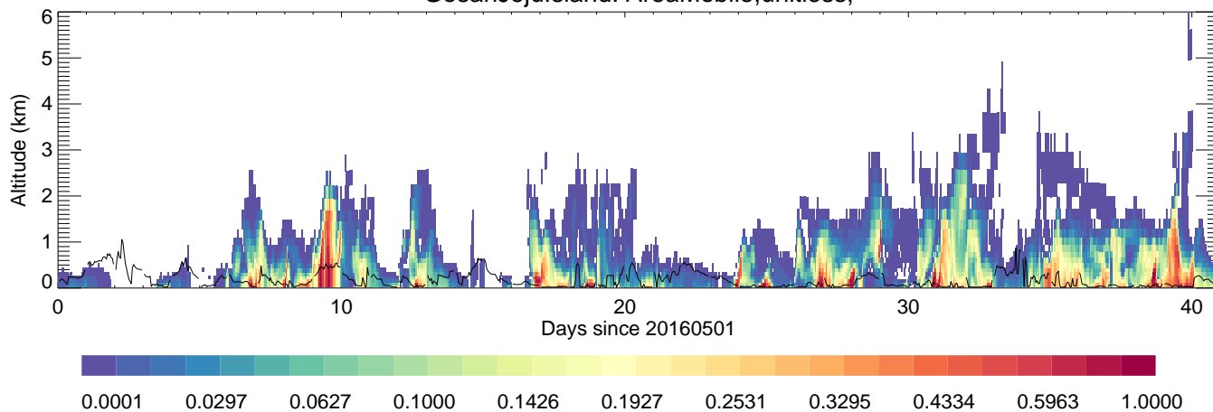
GosanJejulsland: AreaMobile,unitless,
