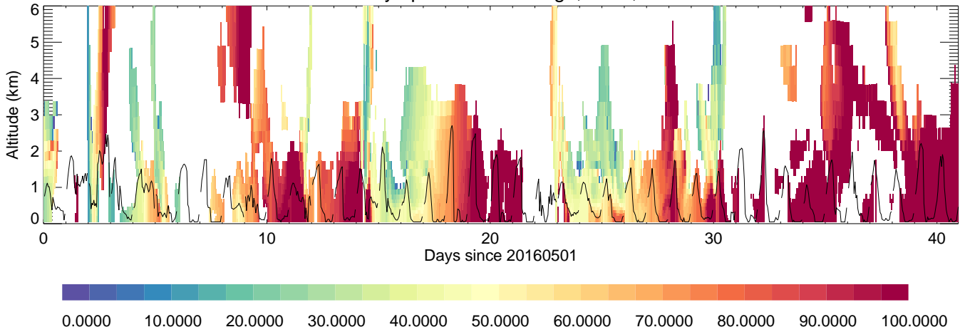
OlympicPark: RH,%,
