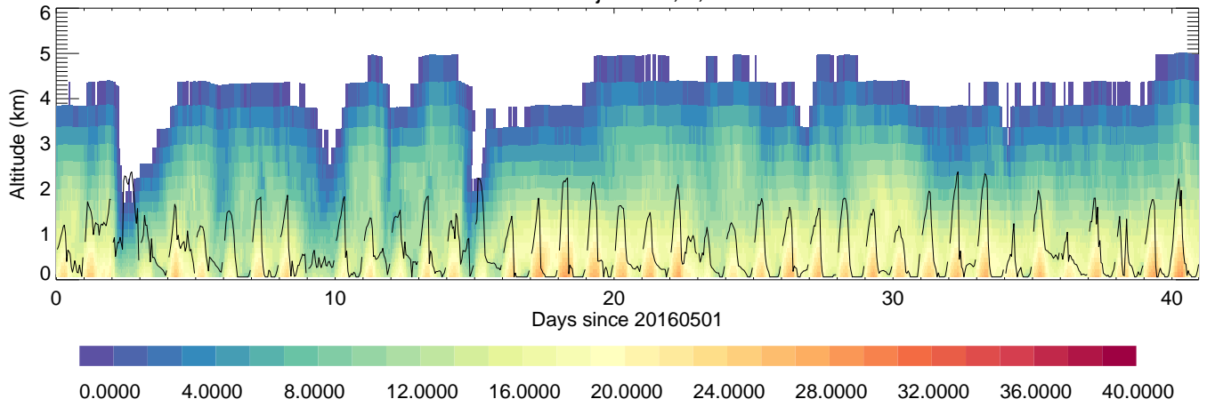
Daejeon: T,C,
