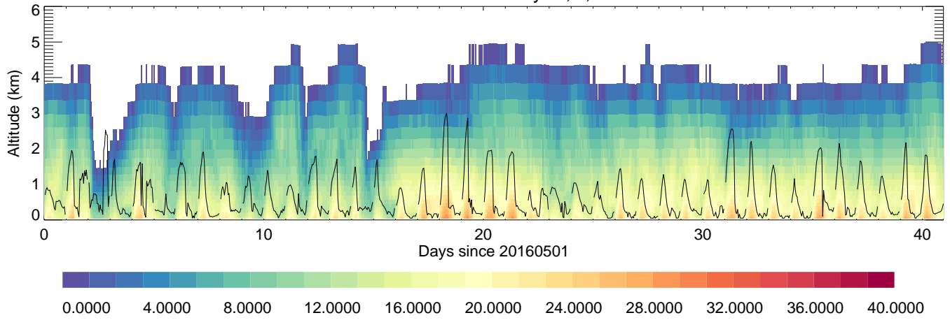
YonseiUniversity: T,C,
