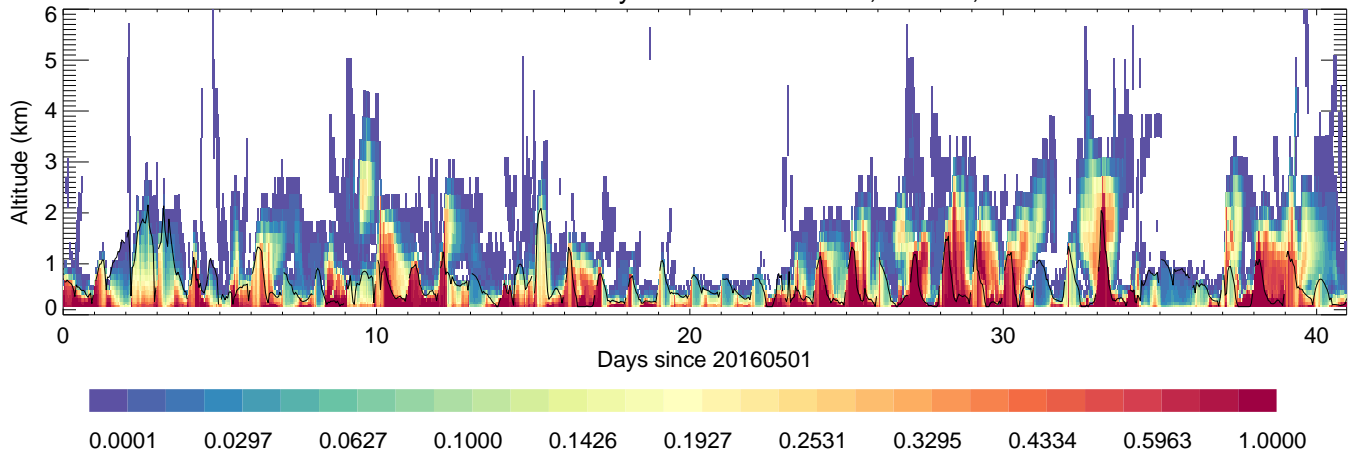
PusanUniversityBusan: AreaMobile,unitless,
