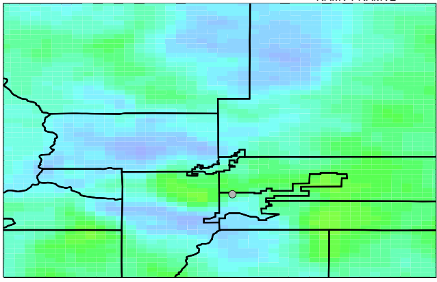
Difference O3 Surface
