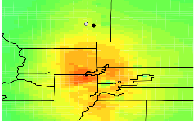
wrfout_d02_2014-07-10_21:00:00_NAMV2
