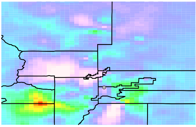
Difference CO Surface
