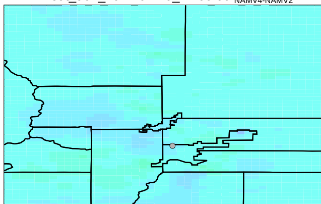
Difference C2H4 Surface
