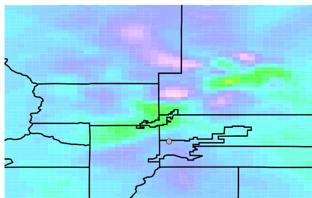
Difference C2H6 Surface
