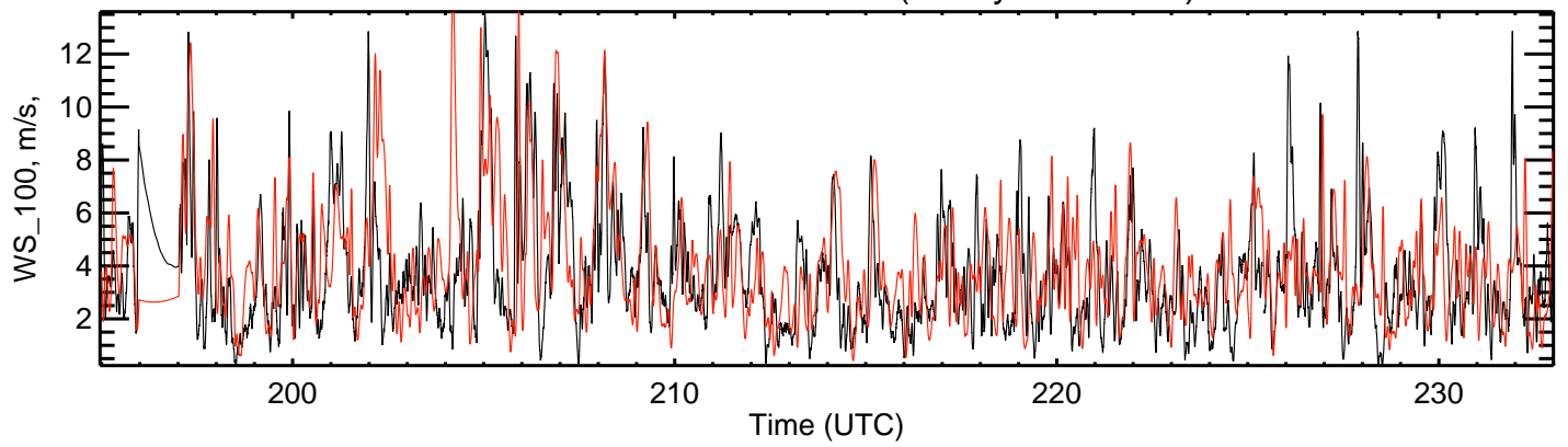
BAO Wind Measurements (hourly smoothed)
