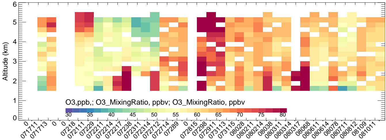
FortCollins BTXv2ECMWFV4mozmozaicRedMobTUVscale-
