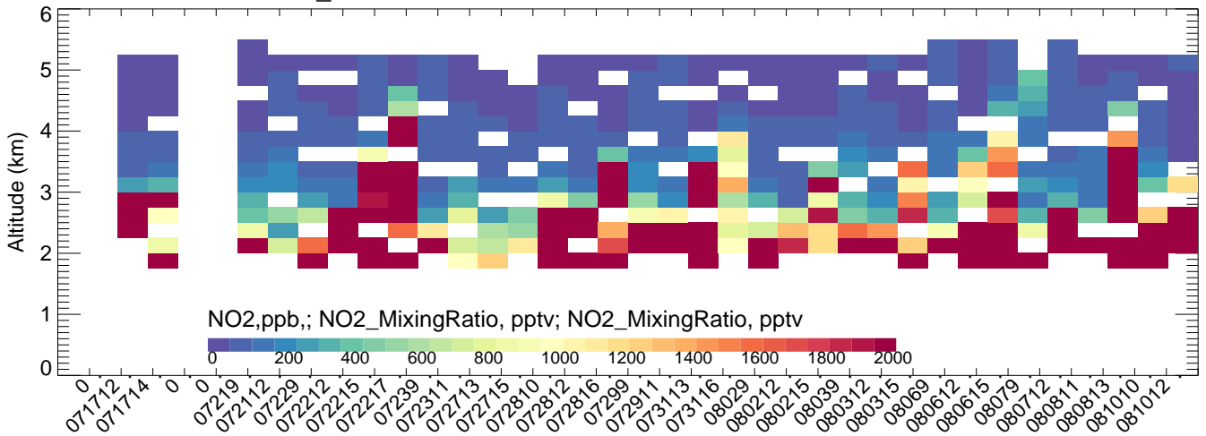
NREL_Golden CMAQ
