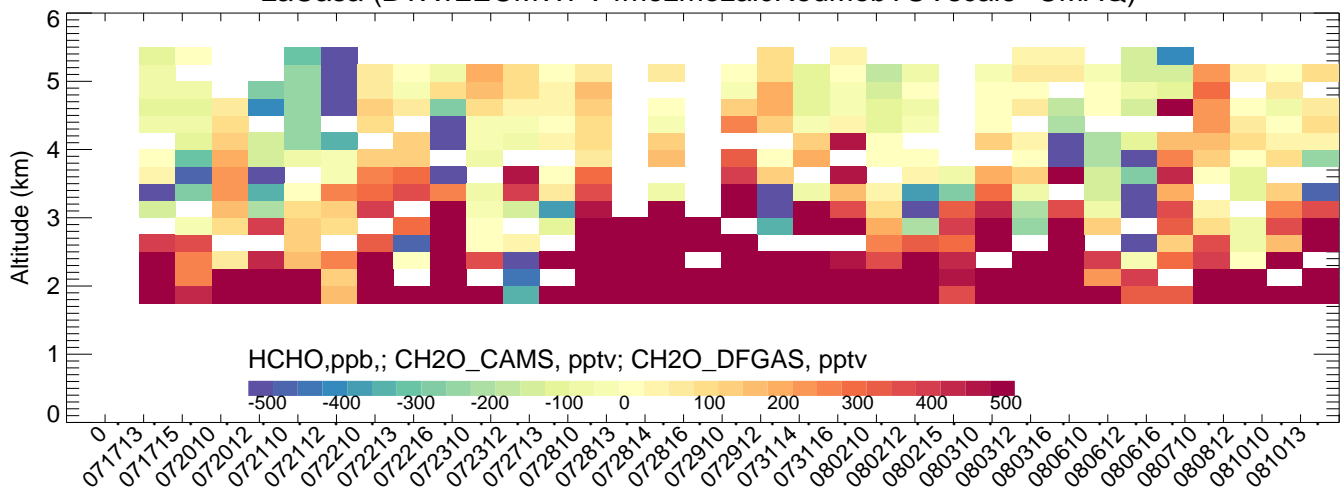
LaCasa (BTXv2ECMWFV4mozmozaicRedMobTUVscale--CMAQ)
