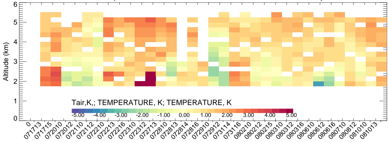
LaCasa (CMAQ-Obs)
