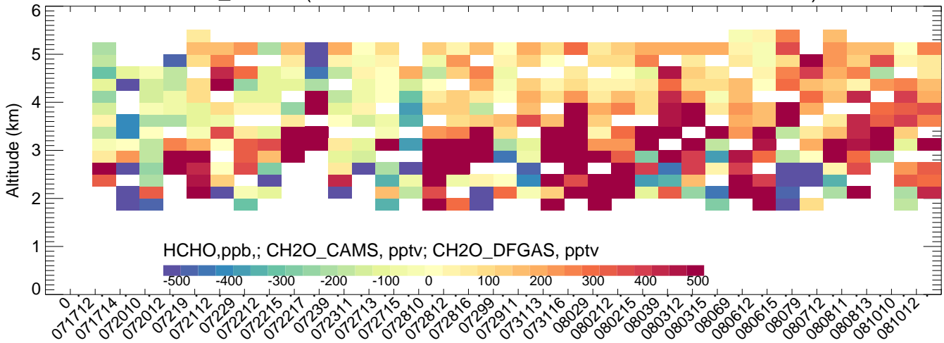
NREL_Golden (CMAQ-Obs)
