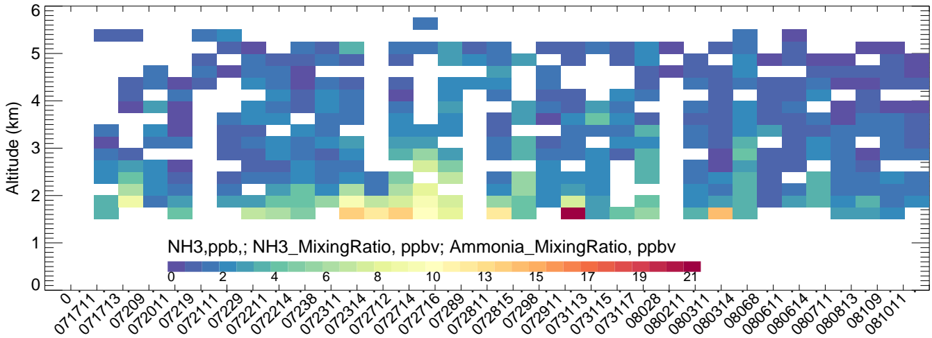
Platteville BTXv2ECMWFV4mozmozaicRedMobTUVscale-
