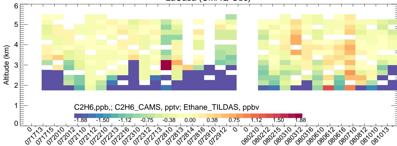
LaCasa (BTXv2ECMWFV4mozmozaicRedMobTUVscale--CMAQ)
