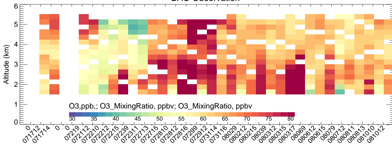
BAO BTXv2ECMWFV4mozmozaicRedMobTUVscale-
