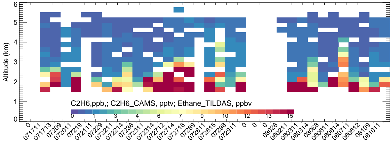
Platteville BTXv2ECMWFV4mozmozaicRedMobTUVscale-
