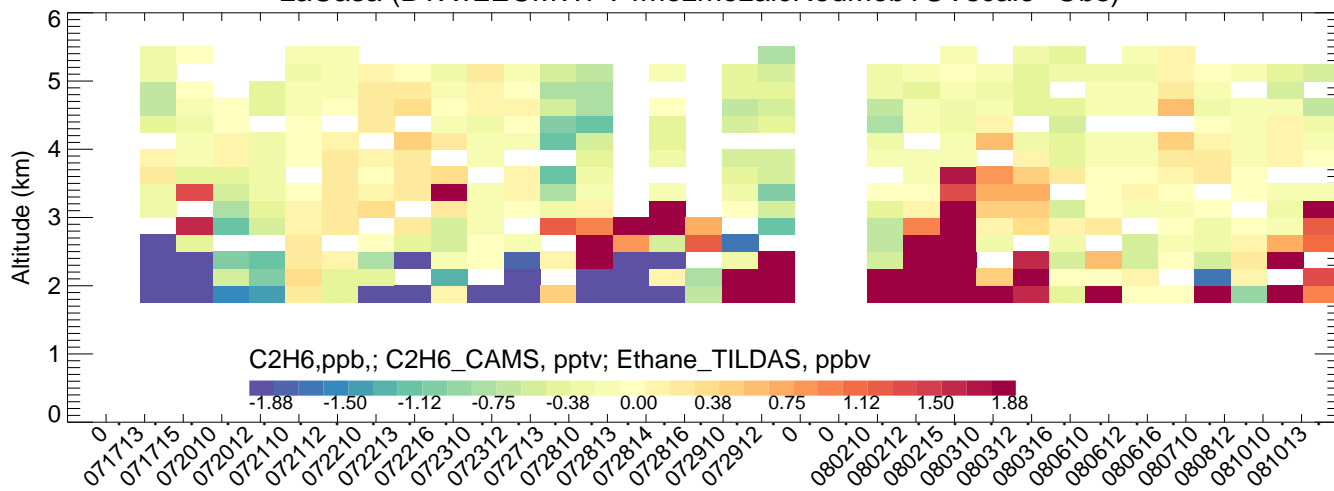
LaCasa (CMAQ-Obs)
