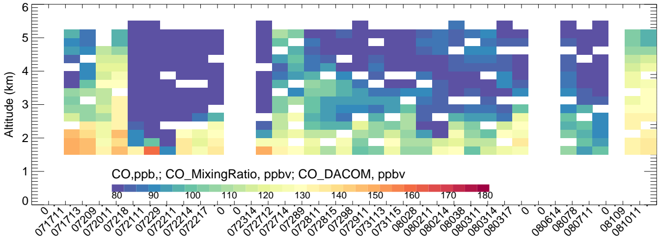
FortCollins BTXv2ECMWFV4mozmozaicRedMobTUVscale-
