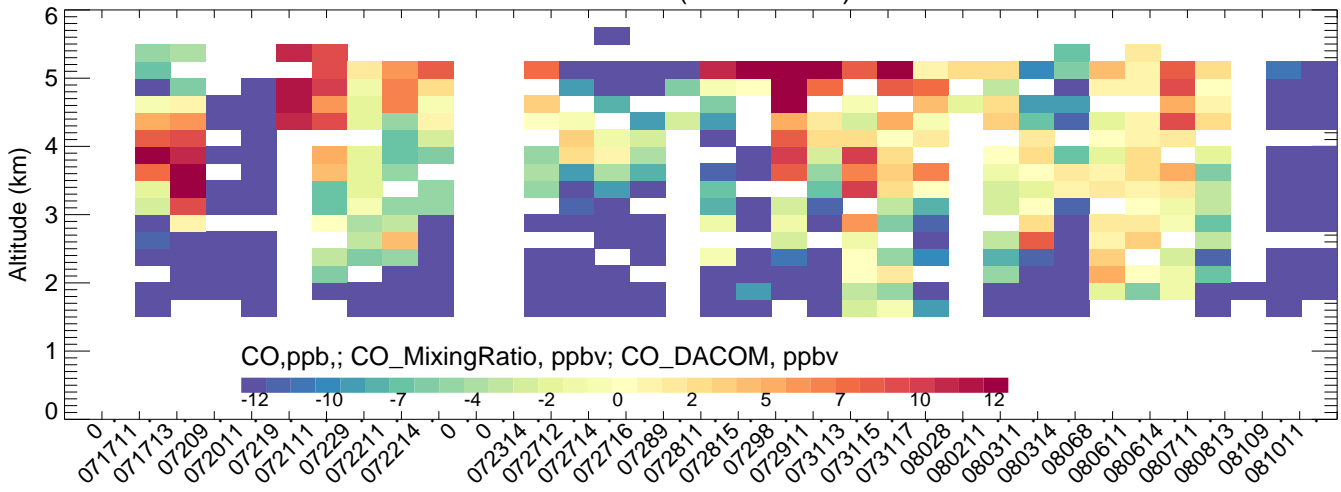
Platteville (BTXv2ECMWFV4mozmozaicRedMobTUVscale--CMAQ)
