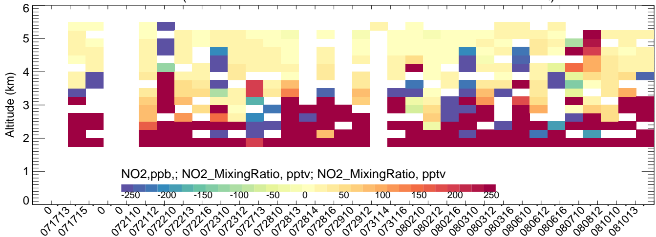
LaCasa (BTXv2ECMWFV4mozmozaicRedMobTUVscale--CMAQ)
