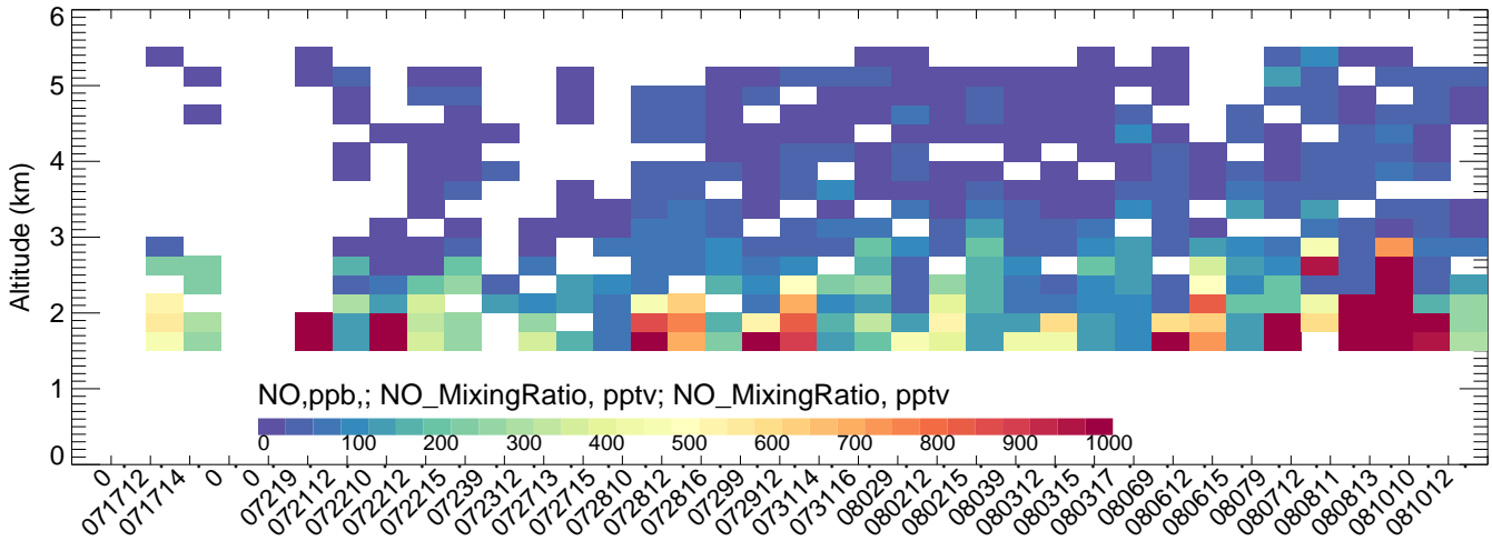
BAO BTXv2ECMWFV4mozmozaicRedMobTUVscale-
