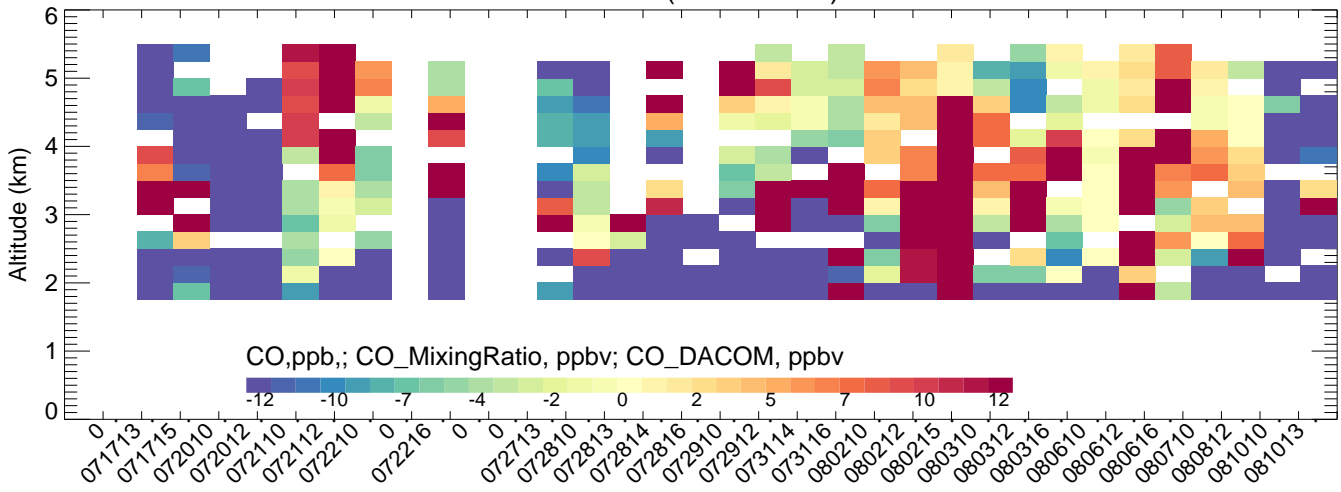
LaCasa (BTXv2ECMWFV4mozmozaicRedMobTUVscale--CMAQ)
