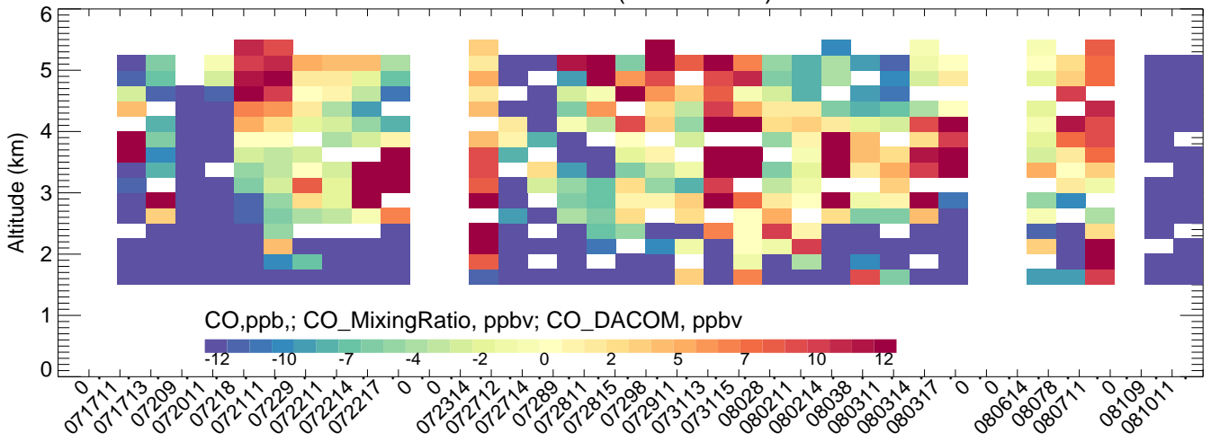
FortCollins (BTXv2ECMWFV4mozmozaicRedMobTUVscale--CMAQ)
