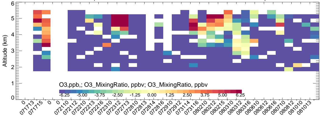
LaCasa (CMAQ-Obs)
