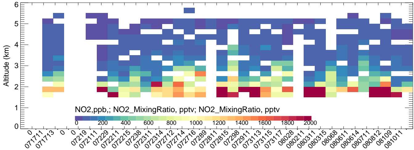
Platteville BTXv2ECMWFV4mozmozaicRedMobTUVscale-
