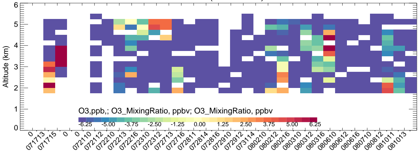
Chatfield (BTXv2ECMWFV4mozmozaicRedMobTUVscale--CMAQ)
