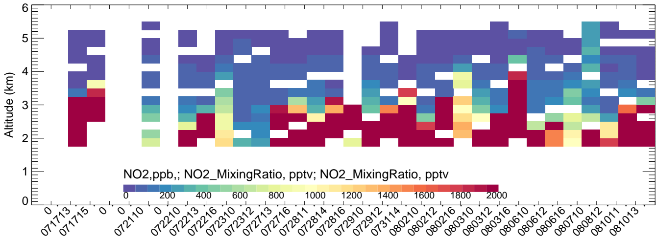
Chatfield CMAQ
