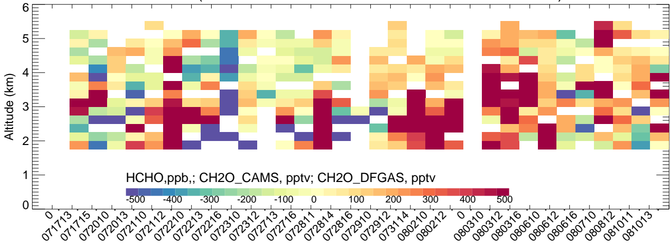
Chatfield (CMAQ-Obs)
