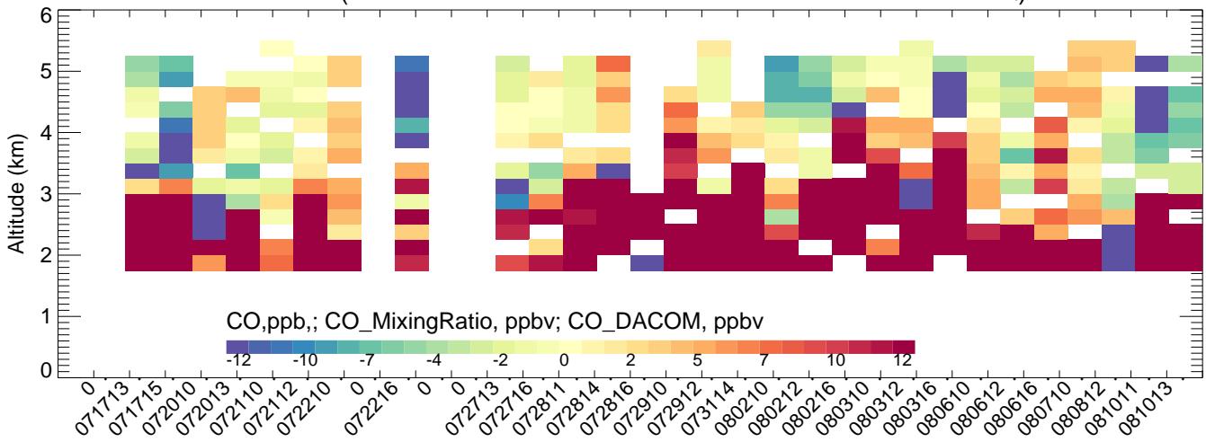
Chatfield (BTXv2ECMWFV4mozmozaicRedMobTUVscale--CMAQ)
