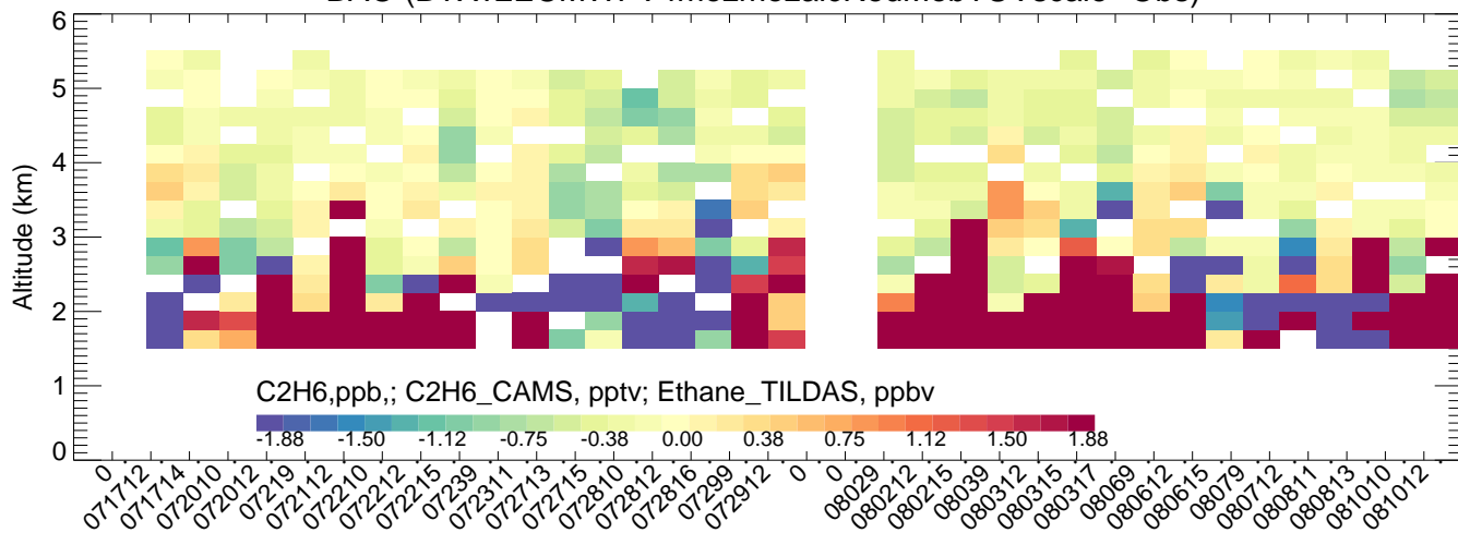
BAO (CMAQ-Obs)
