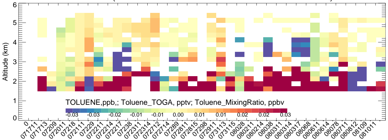
FortCollins (BTXv2ECMWFV4mozmozaicRedMobTUVscale--CMAQ)
