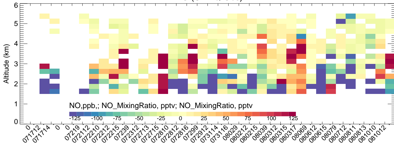
BAO (BTXv2ECMWFV4mozmozaicRedMobTUVscale--CMAQ)
