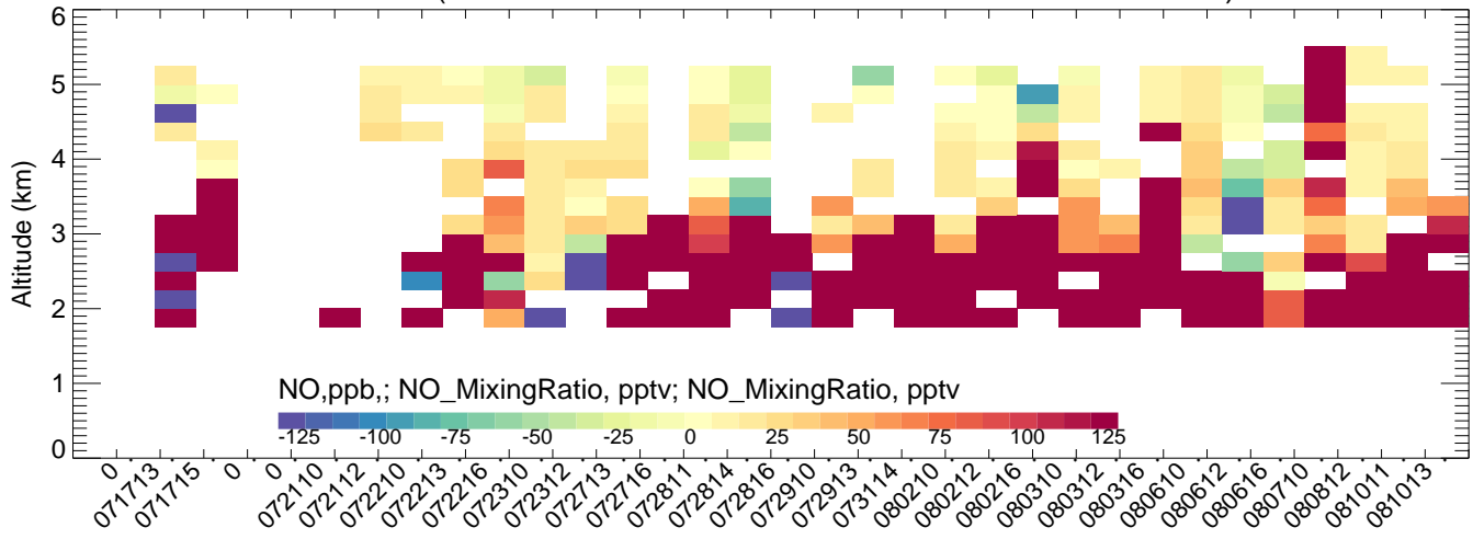
Chatfield (CMAQ-Obs)
