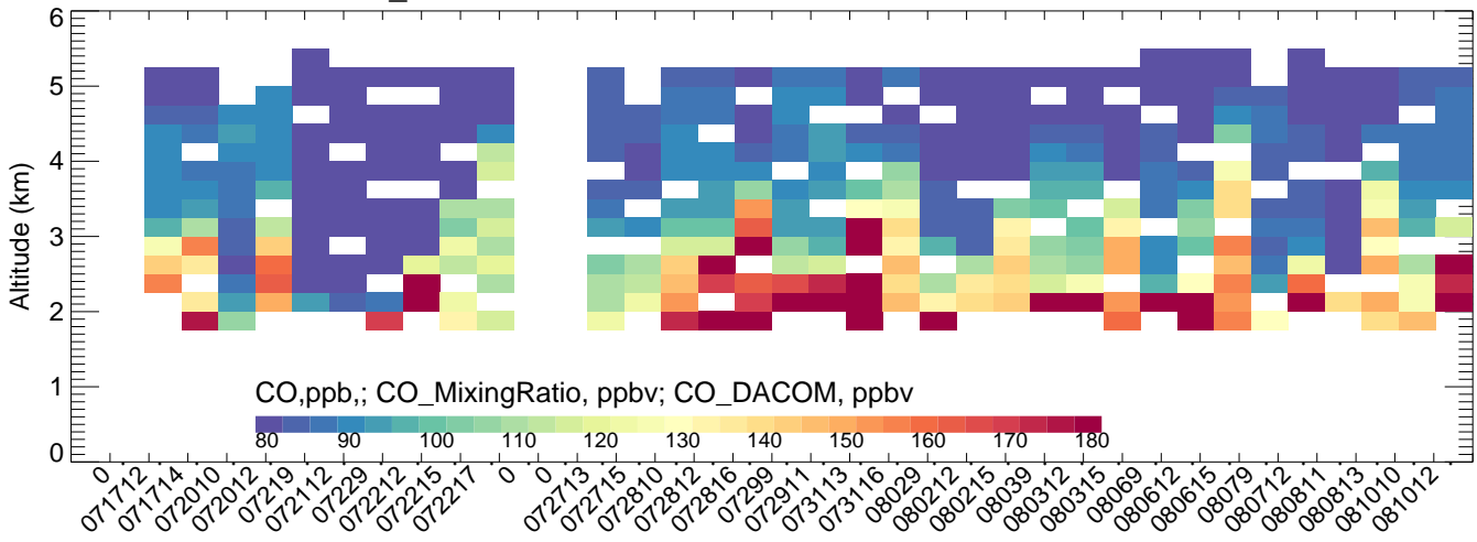
NREL_Golden CMAQ
