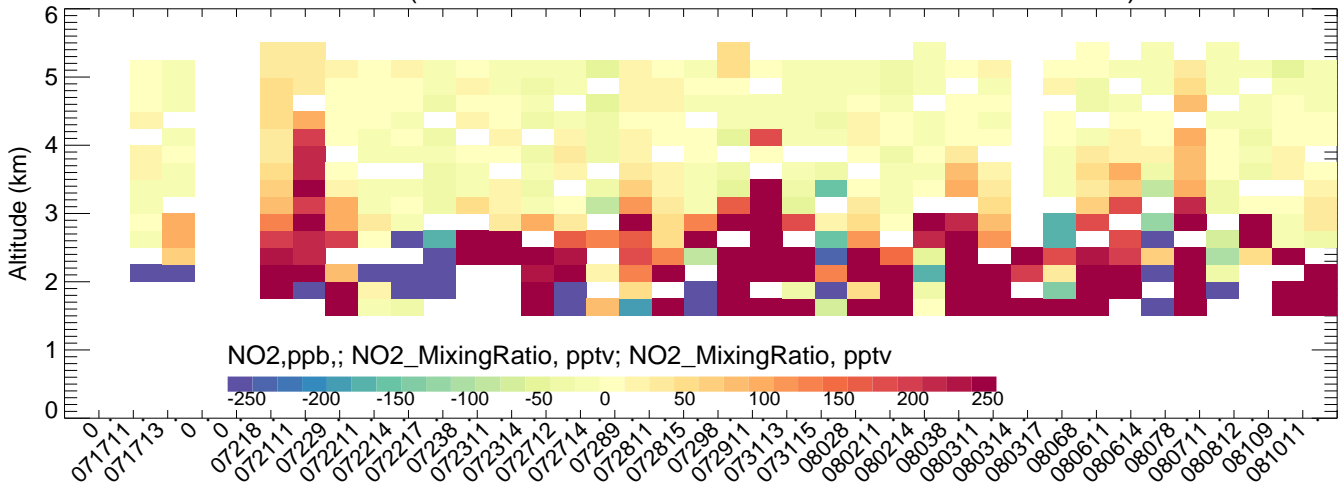
FortCollins (CMAQ-Obs)
