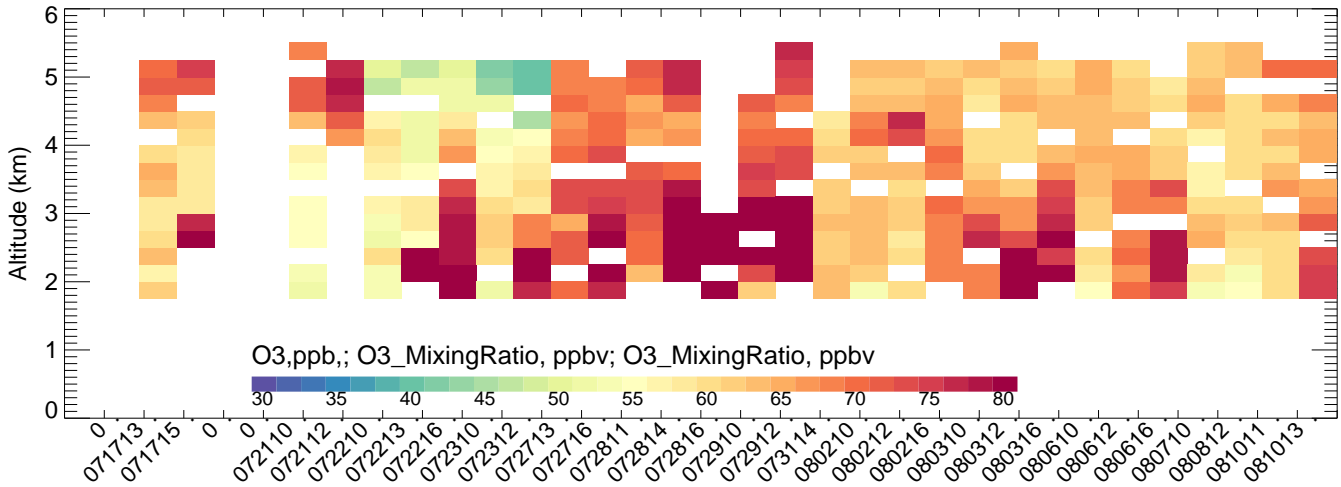
Chatfield BTXv2ECMWFV4mozmozaicRedMobTUVscale-
