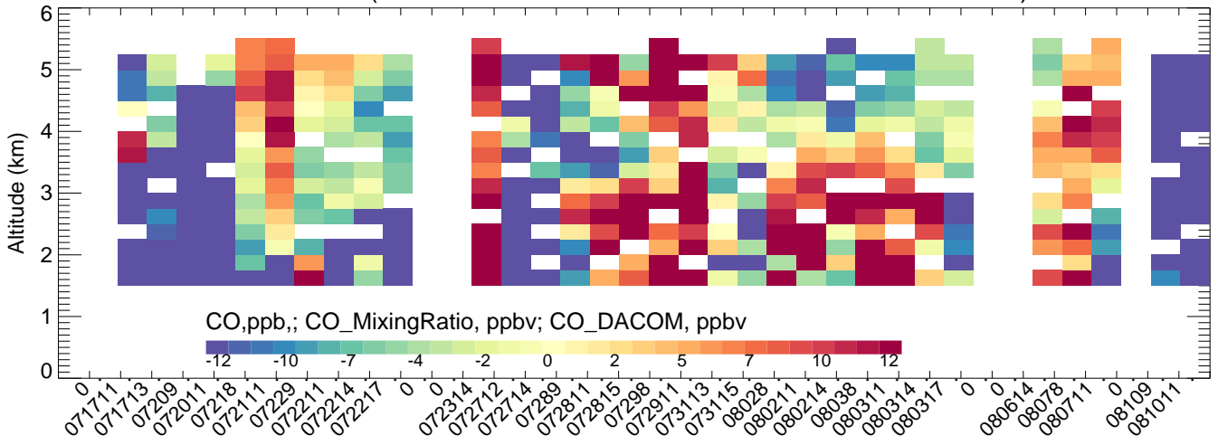
FortCollins (CMAQ-Obs)
