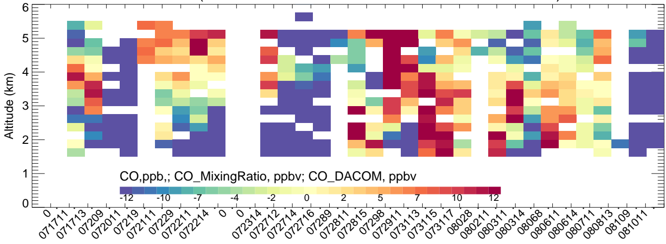
Platteville (CMAQ-Obs)
