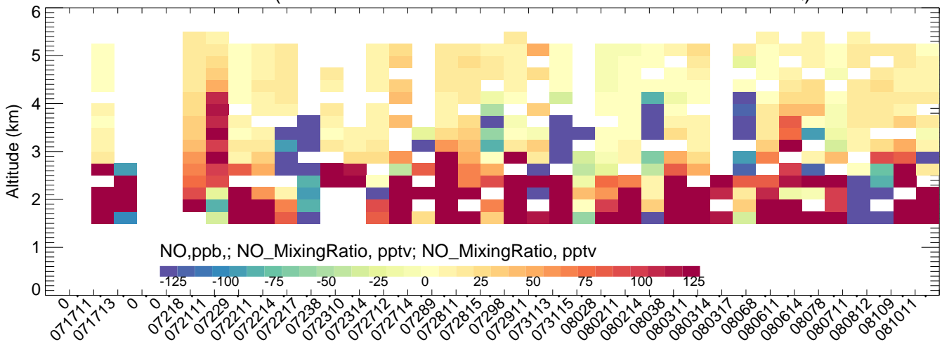
FortCollins (BTXv2ECMWFV4mozmozaicRedMobTUVscale--CMAQ)
