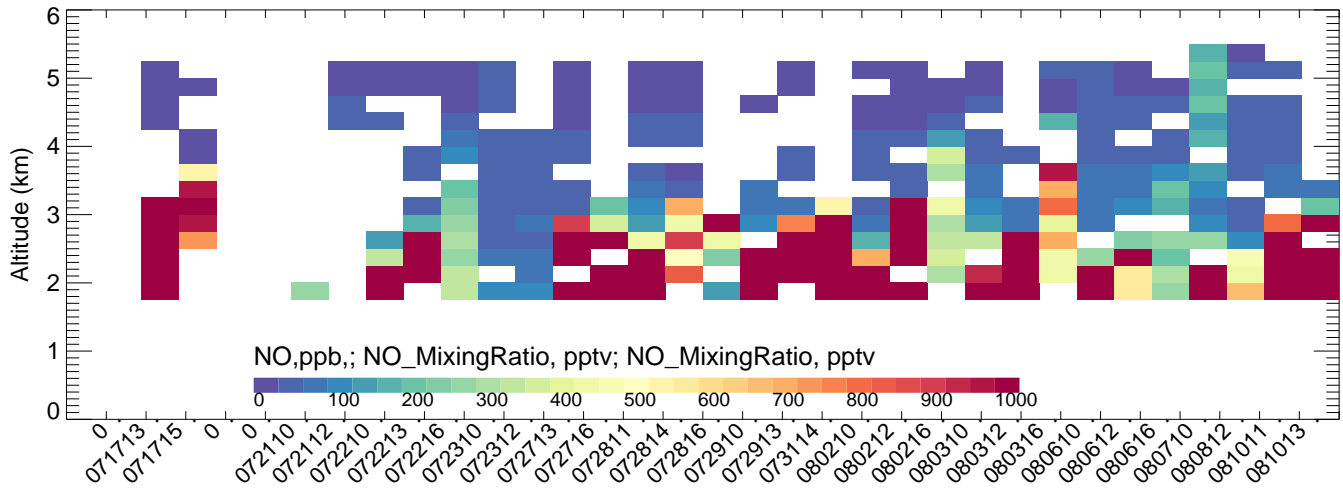
Chatfield CMAQ
