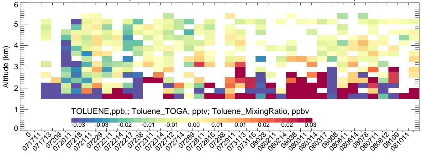
FortCollins (CMAQ-Obs)
