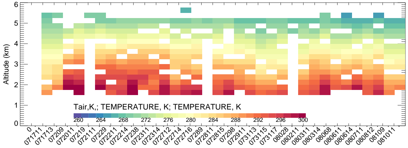
Platteville BTXv2ECMWFV4mozmozaicRedMobTUVscale-
