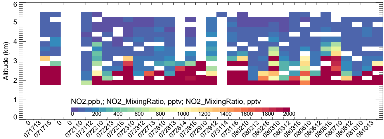
LaCasa BTXv2ECMWFV4mozmozaicRedMobTUVscale-
