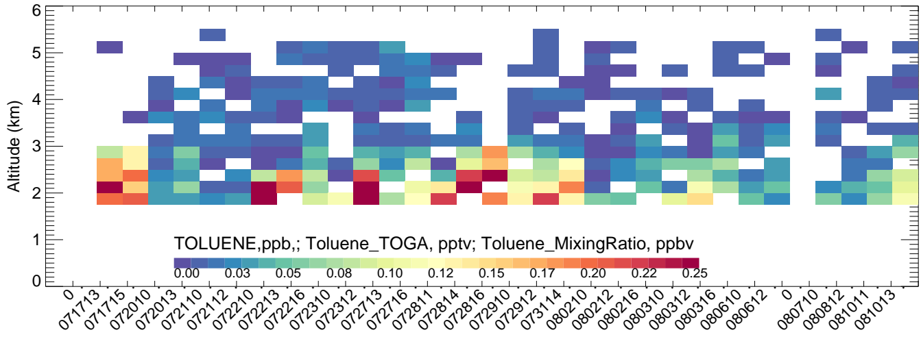
Chatfield BTXv2ECMWFV4mozmozaicRedMobTUVscale-
