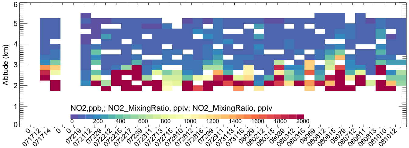
NREL_Golden BTXv2ECMWFV4mozmozaicRedMobTUVscale-
