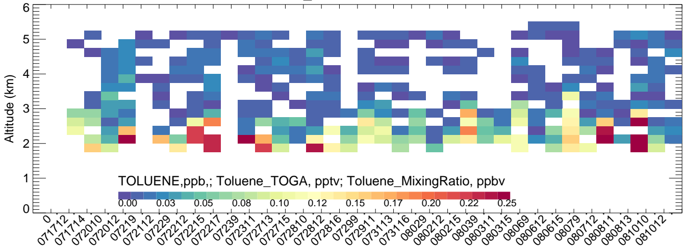
NREL_Golden BTXv2ECMWFV4mozmozaicRedMobTUVscale-
