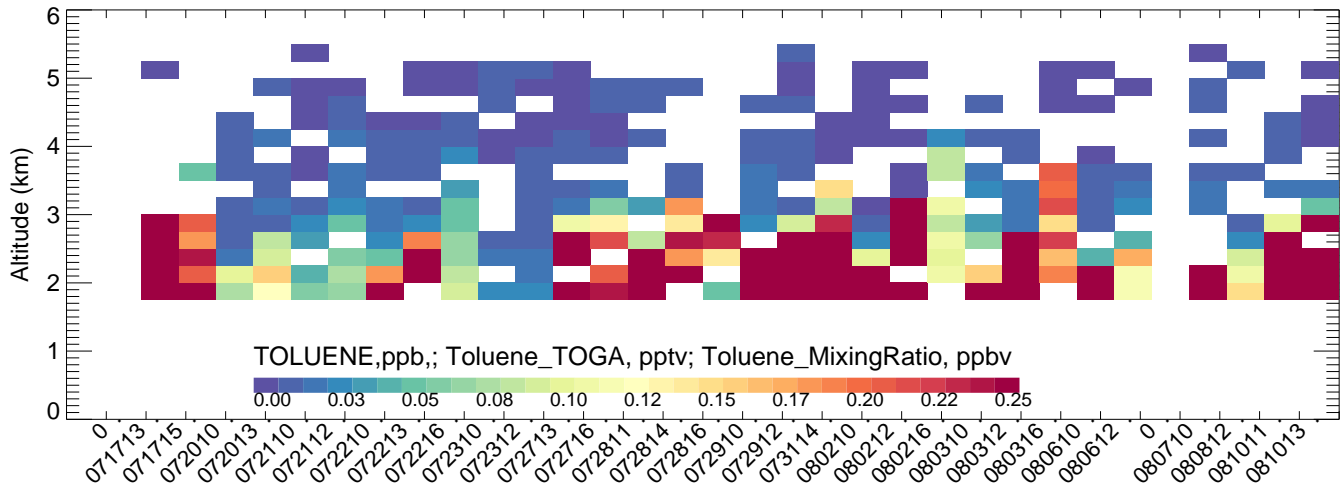
Chatfield CMAQ
