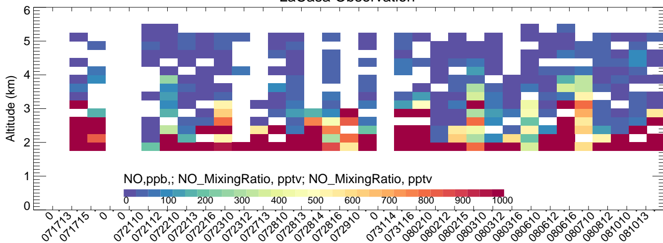
LaCasa BTXv2ECMWFV4mozmozaicRedMobTUVscale-
