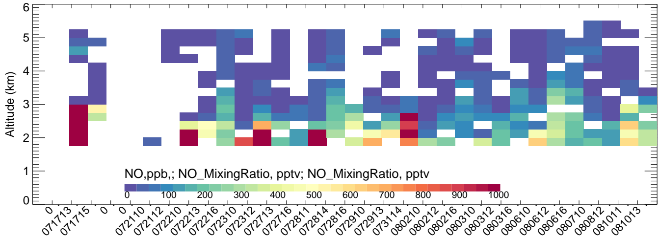
Chatfield BTXv2ECMWFV4mozmozaicRedMobTUVscale-
