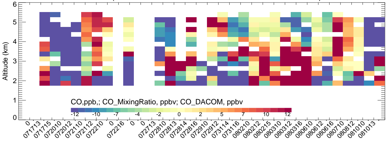
LaCasa (CMAQ-Obs)
