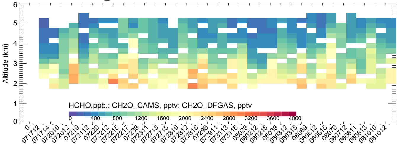
NREL_Golden CMAQ
