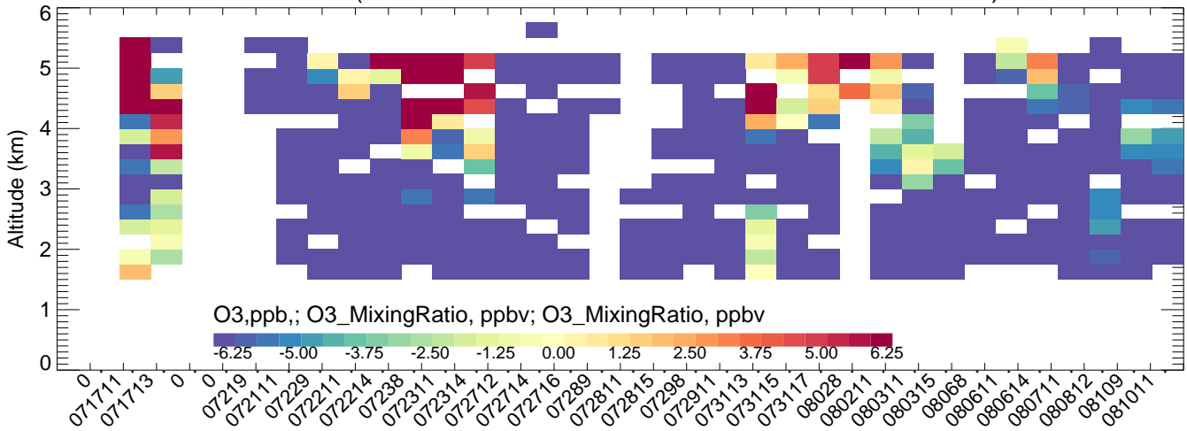
Platteville (CMAQ-Obs)
