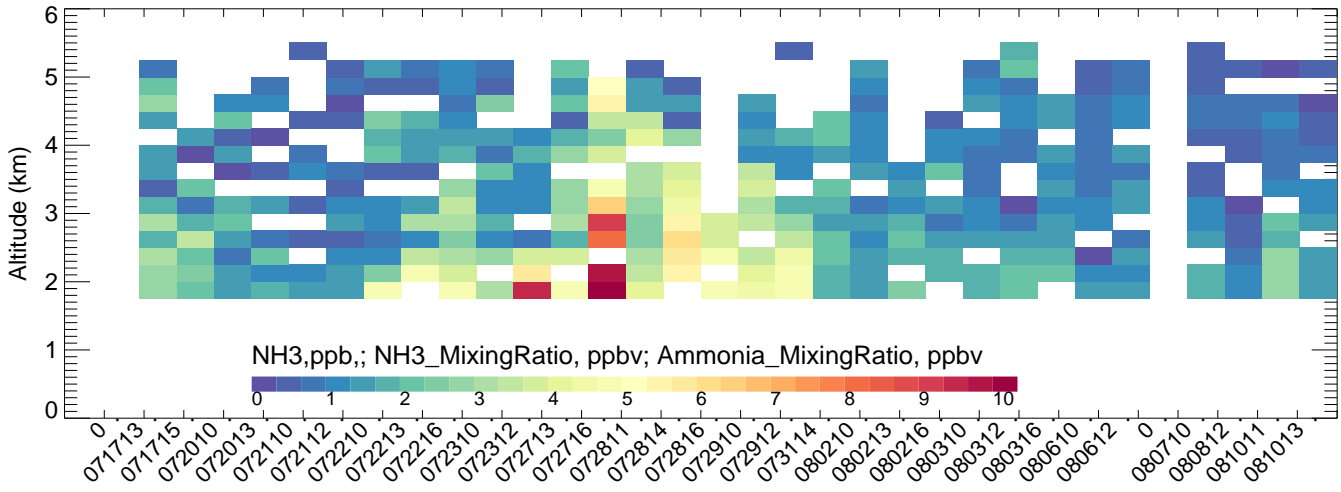
Chatfield BTXv2ECMWFV4mozmozaicRedMobTUVscale-
