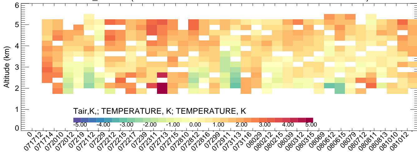
NREL_Golden (BTXv2ECMWFV4mozmozaicRedMobTUVscale--CMAQ)
