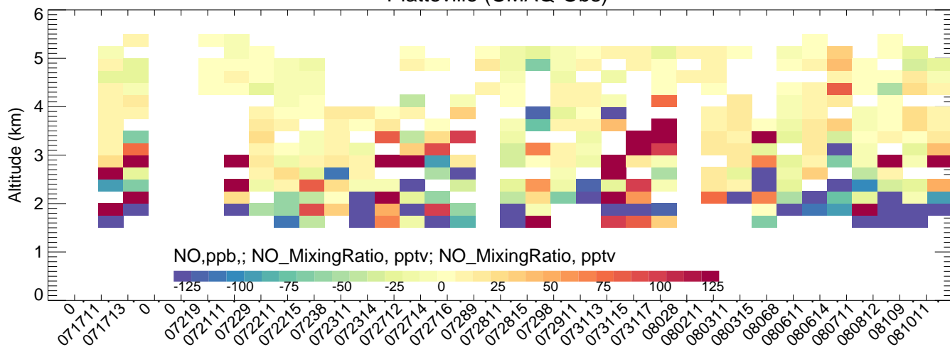
Platteville (BTXv2ECMWFV4mozmozaicRedMobTUVscale--CMAQ)
