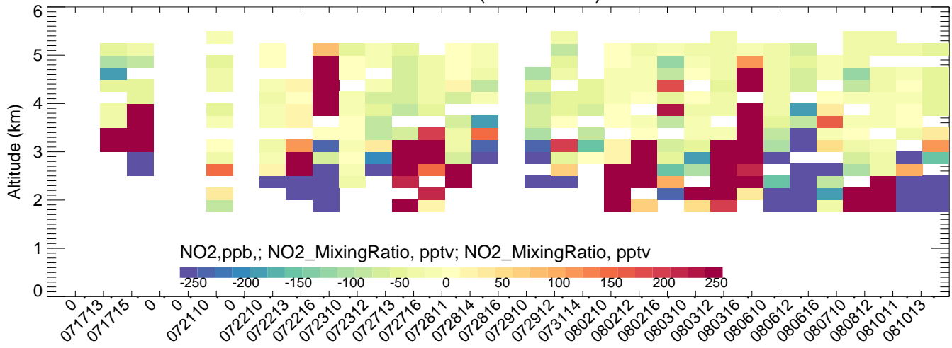
Chatfield (BTXv2ECMWFV4mozmozaicRedMobTUVscale--CMAQ)
