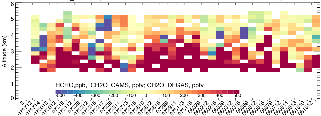
NREL_Golden (BTXv2ECMWFV4mozmozaicRedMobTUVscale--CMAQ)
