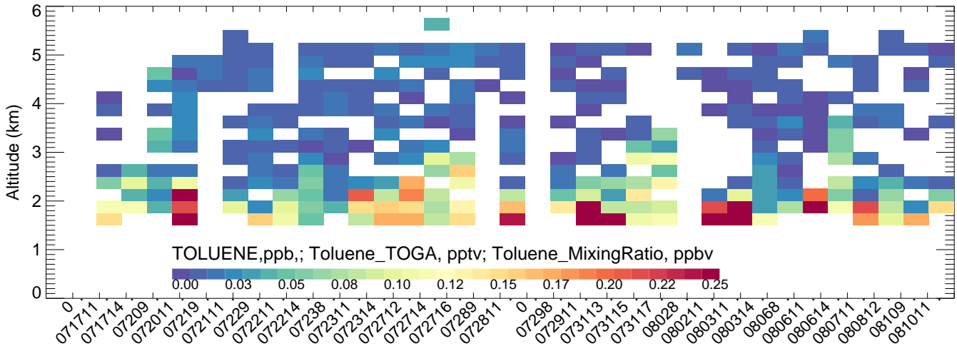
Platteville BTXv2ECMWFV4mozmozaicRedMobTUVscale-
