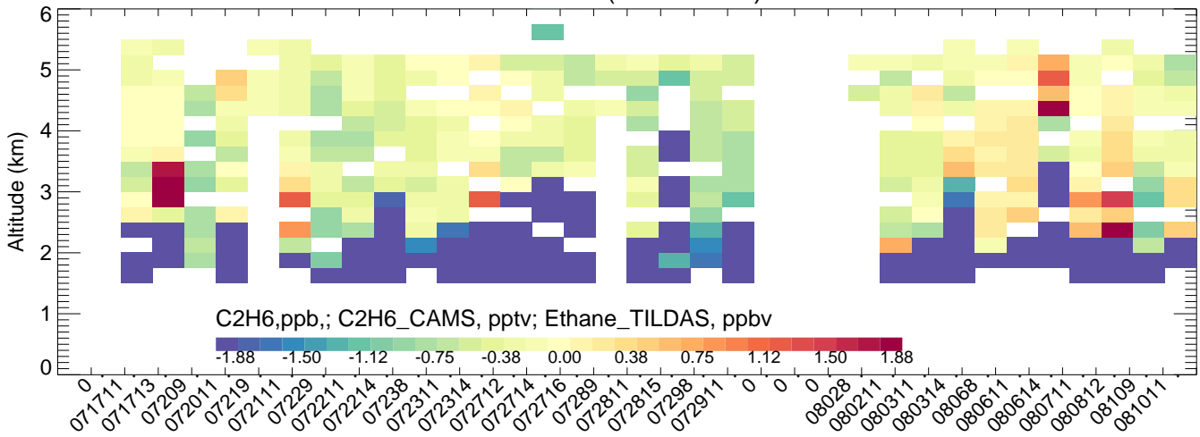
Platteville (BTXv2ECMWFV4mozmozaicRedMobTUVscale--CMAQ)
