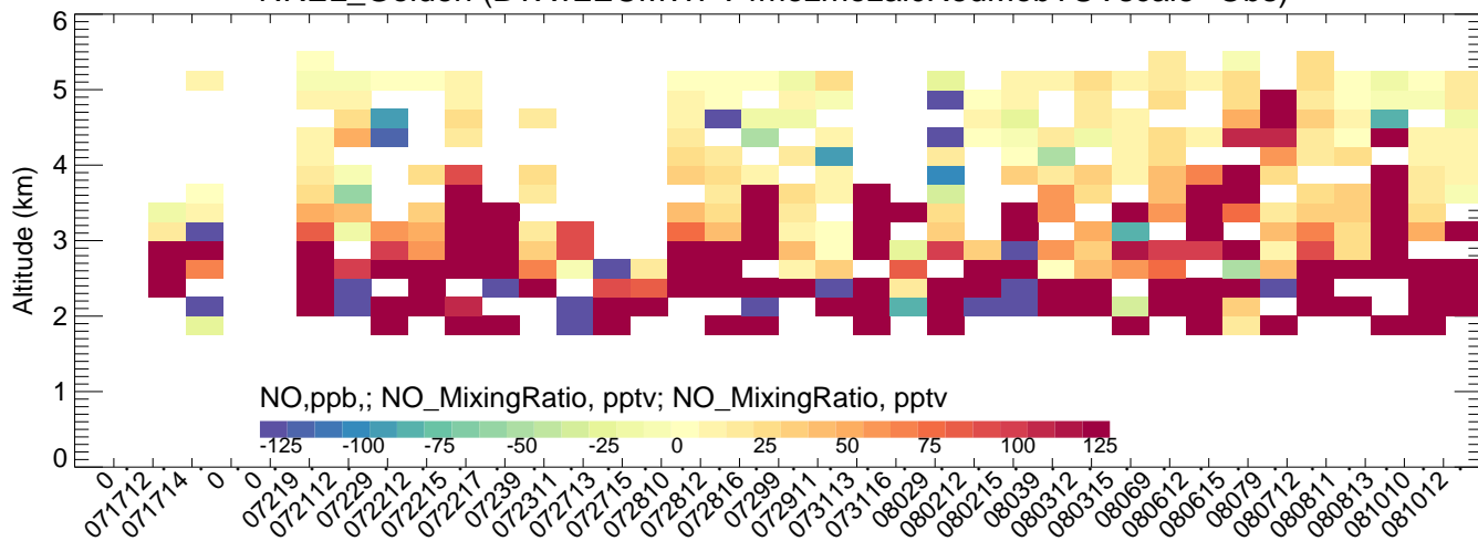
NREL_Golden (CMAQ-Obs)
