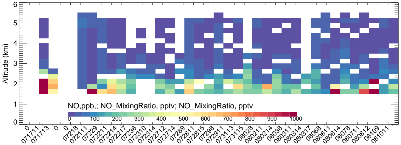
FortCollins BTXv2ECMWFV4mozmozaicRedMobTUVscale-
