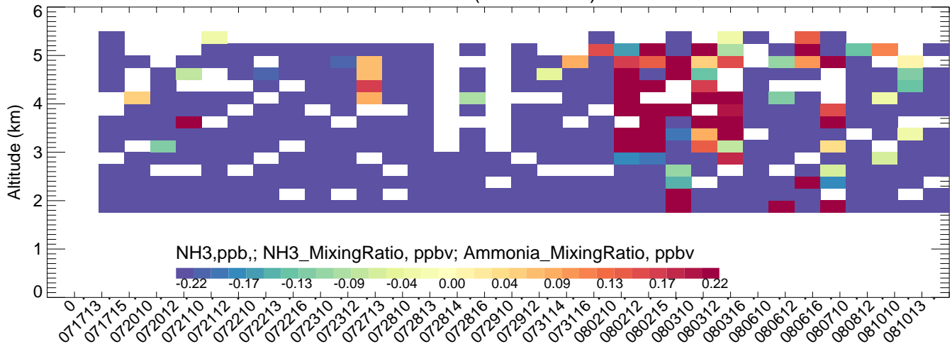
LaCasa (BTXv2ECMWFV4mozmozaicRedMobTUVscale--CMAQ)
