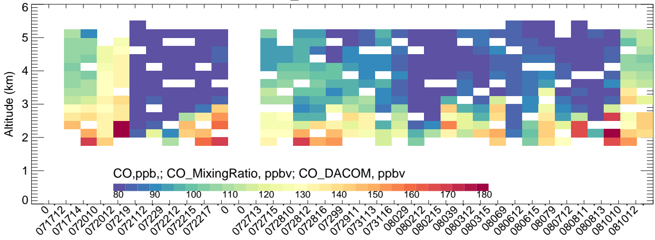
NREL_Golden BTXv2ECMWFV4mozmozaicRedMobTUVscale-
