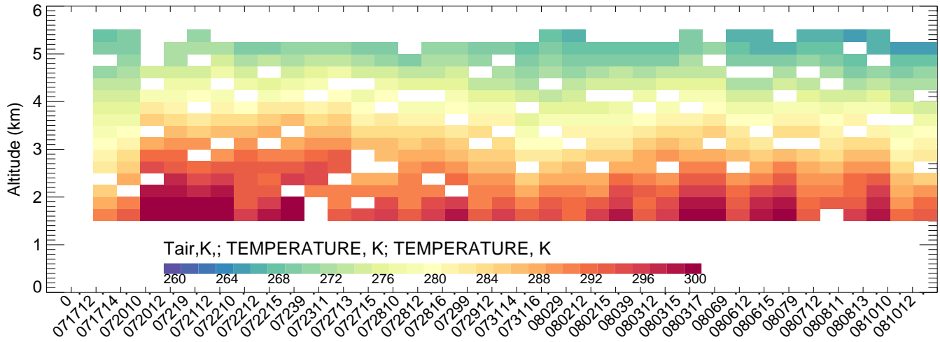
BAO BTXv2ECMWFV4mozmozaicRedMobTUVscale-
