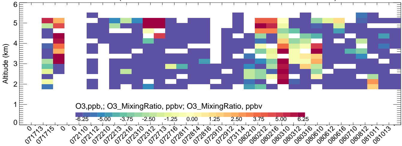
Chatfield (CMAQ-Obs)
