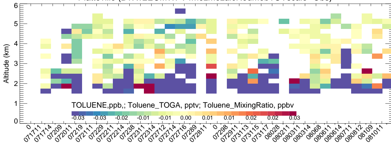
Platteville (CMAQ-Obs)
