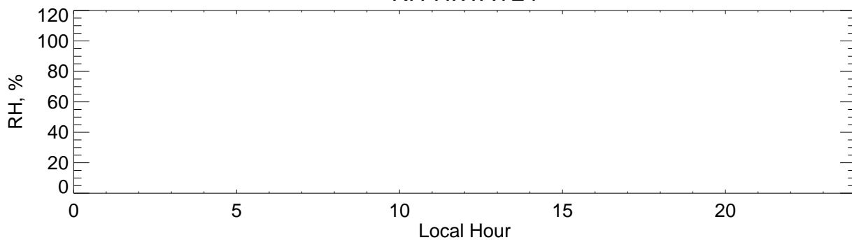
RH-HIWAY24
