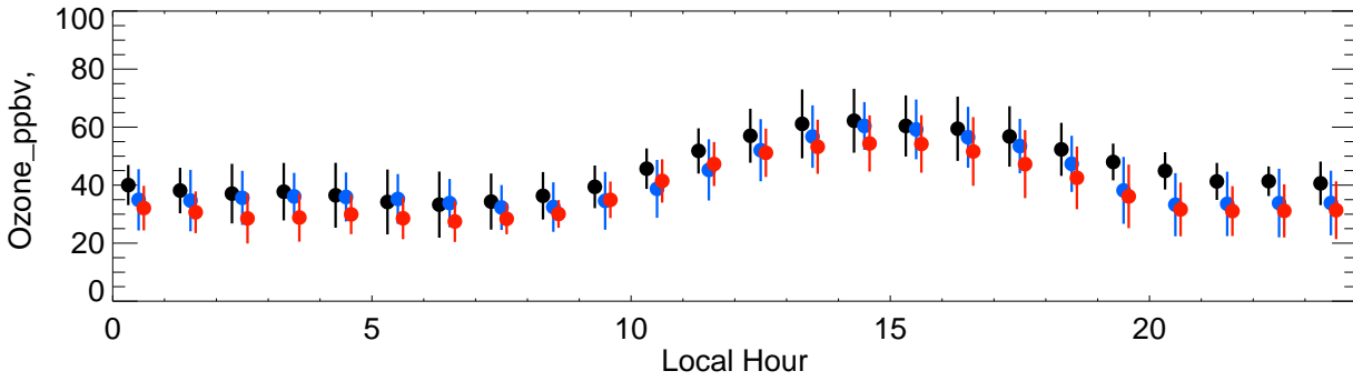
GROUND-NREL-GOLDEN
