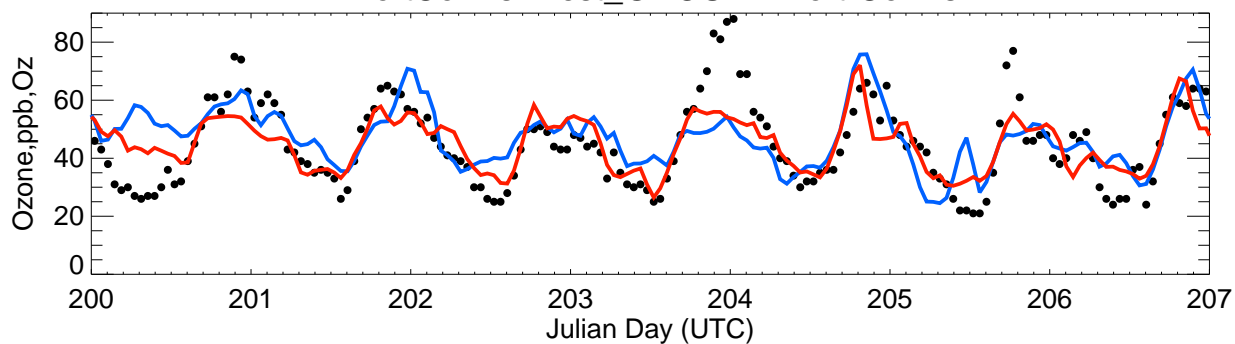
-FortCollins-West_GROUND-Fort-Collins
