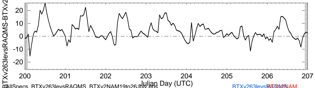
O3-LAYPEAK
