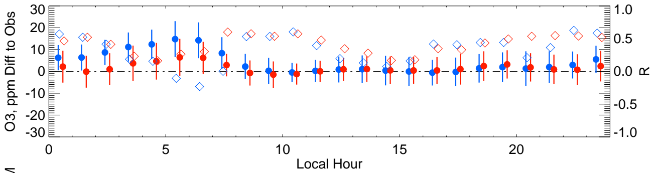
O3-LAYPEAK
