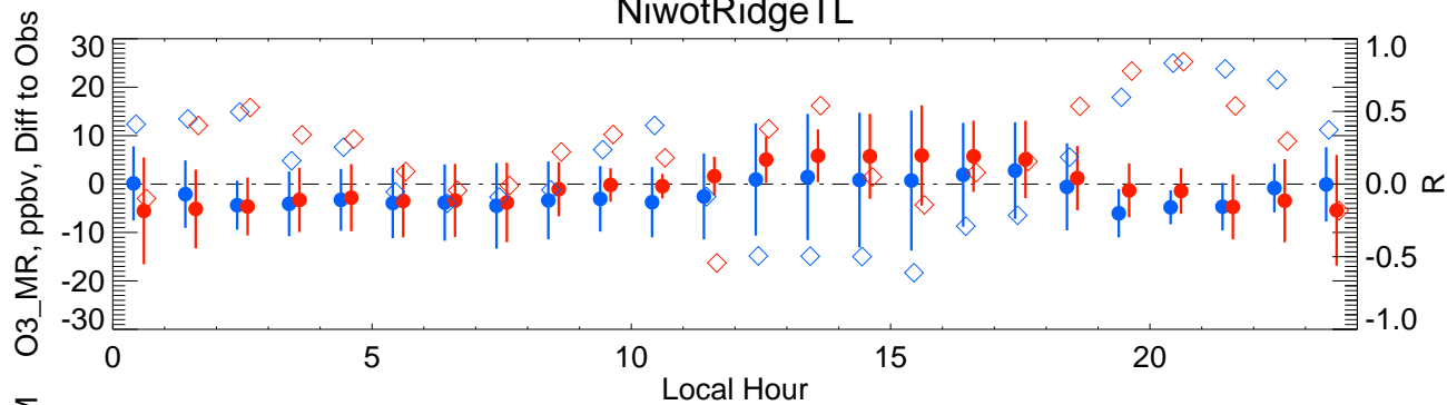
NiwotRidgeTL
