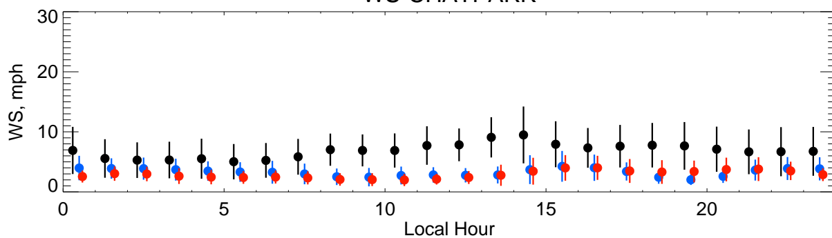
WS-CHATPARK
