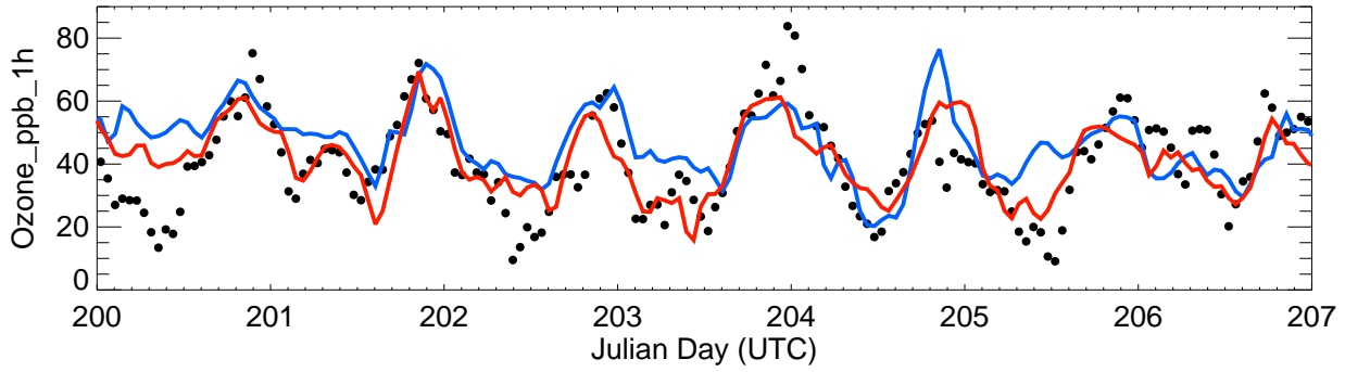
GO3EastBoulder
