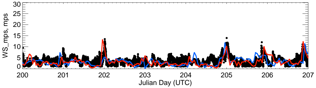
PlattevilleNative
