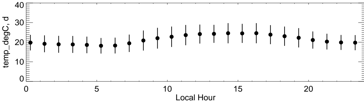
GROUND-NREL-GOLDEN
