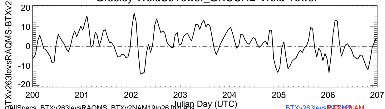
-Greeley-WeldCoTower_GROUND-Weld-Tower
