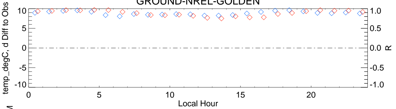
GROUND-NREL-GOLDEN
