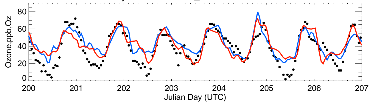
-Greeley-WeldCoTower_GROUND-Weld-Tower
