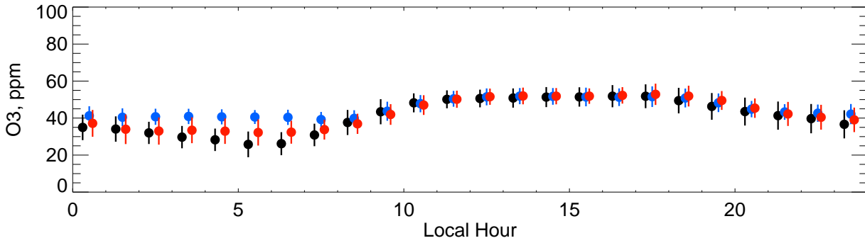
O3-LAYPEAK
