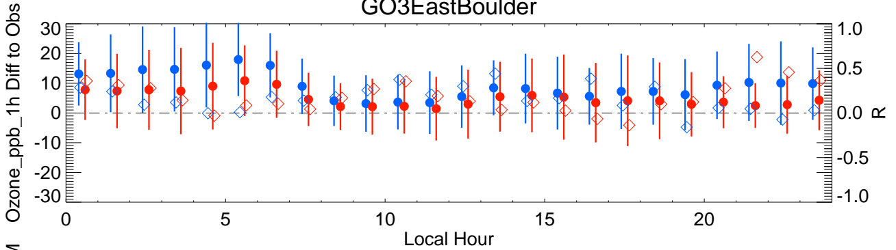
GO3EastBoulder
