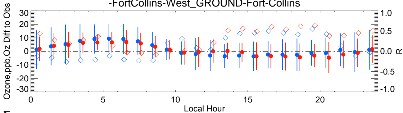
-FortCollins-West_GROUND-Fort-Collins
