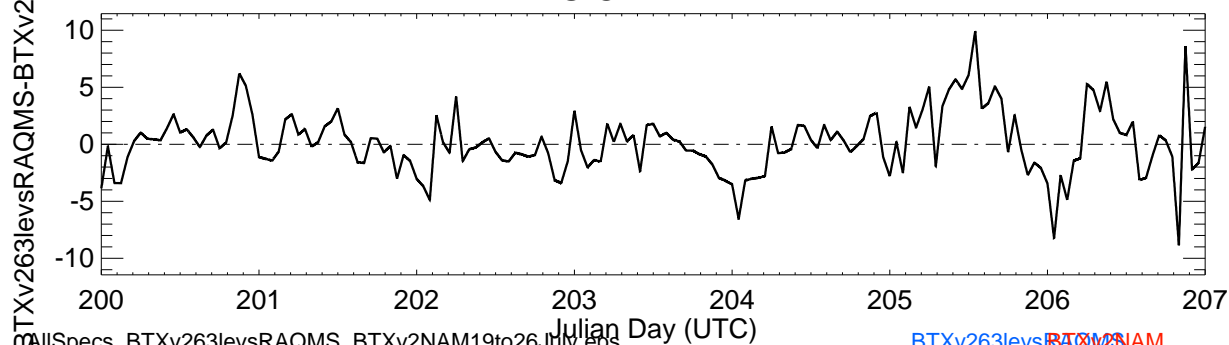
WS-CHATPARK
