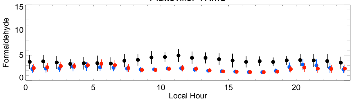
PlattevillePTRMS
