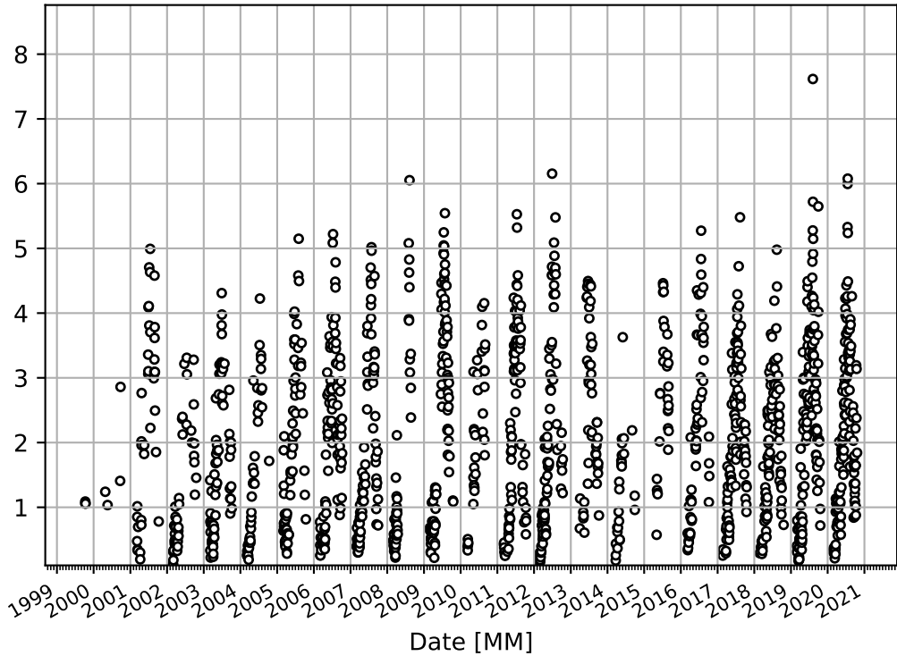
Time Series of Daily Averaged Total Column
