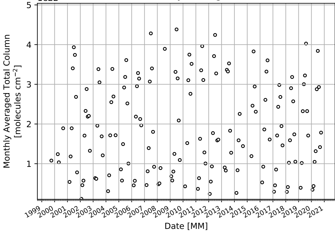
Time Series of Monthly Averaged Total Column
