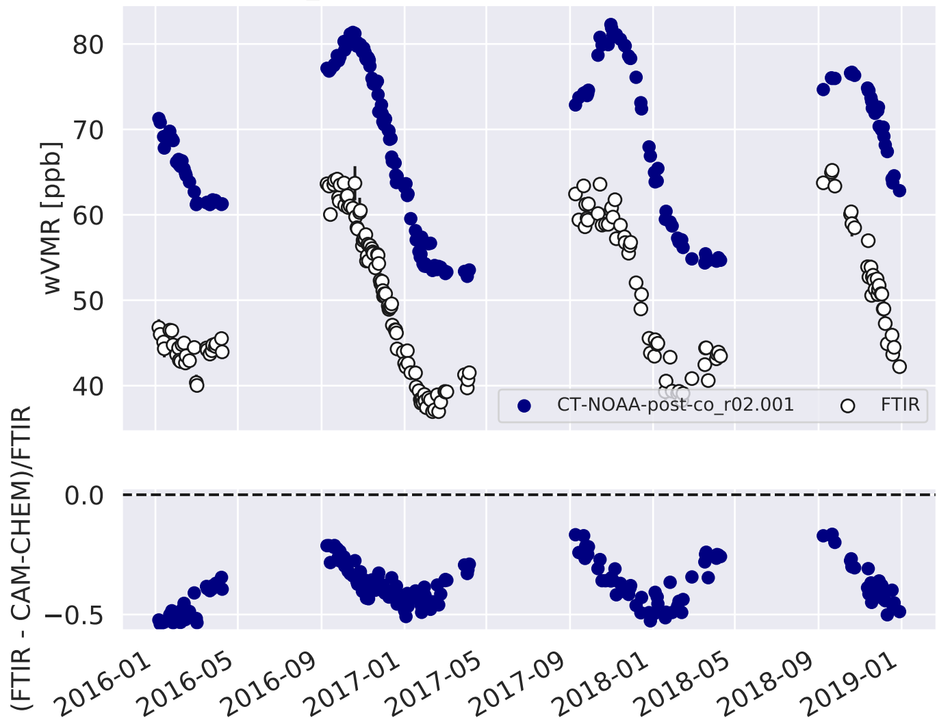
Arrival_Heights (lat:-77.8, lon:166.6, alt:0.2 km)
