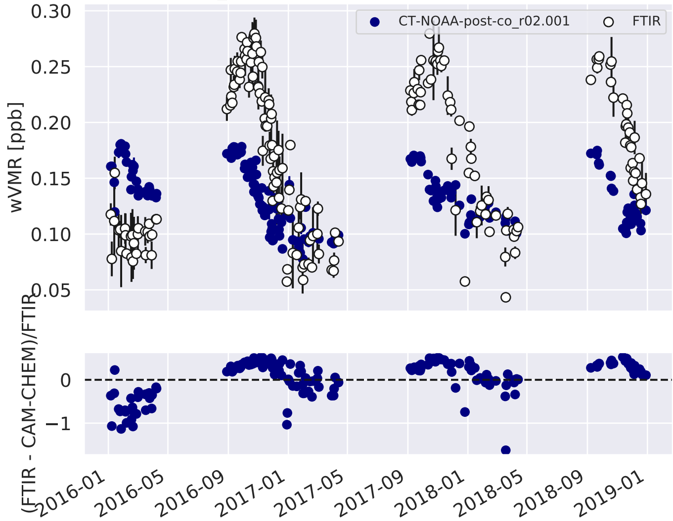
Arrival_Heights (lat:-77.8, lon:166.6, alt:0.2 km)
